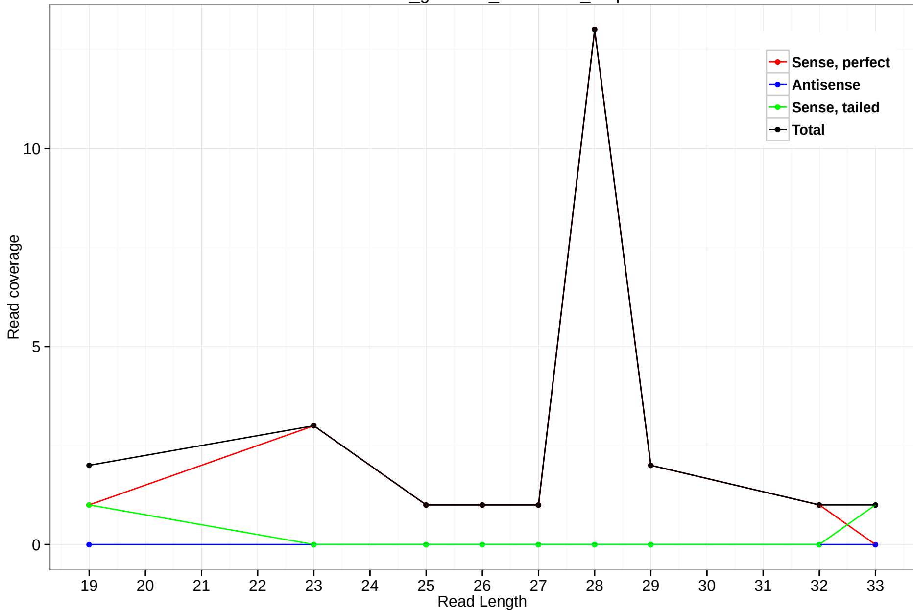
rheMac3_genscan_chr6.1399_5.3p
