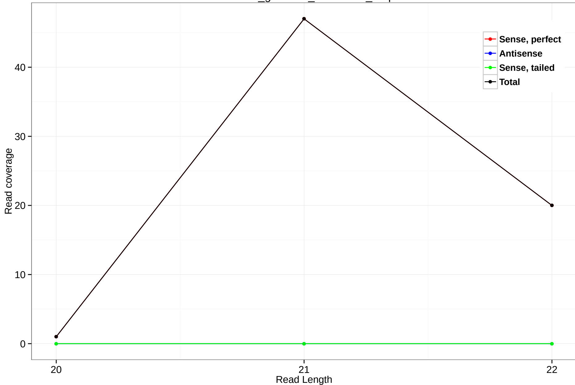
rheMac3_genscan_chr6.1386_1.3p
