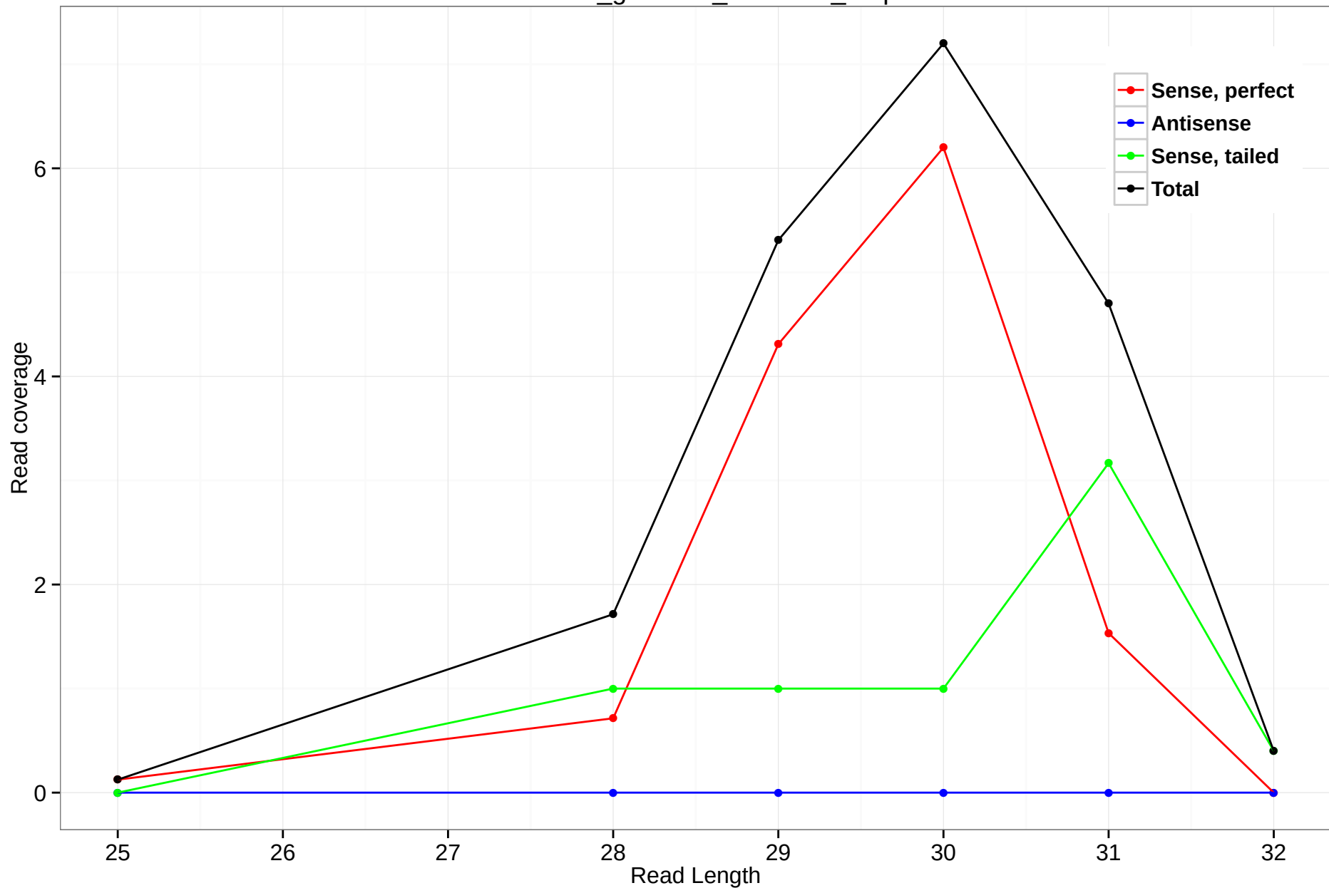
rheMac3_genscan_chr6.133_9.5p
