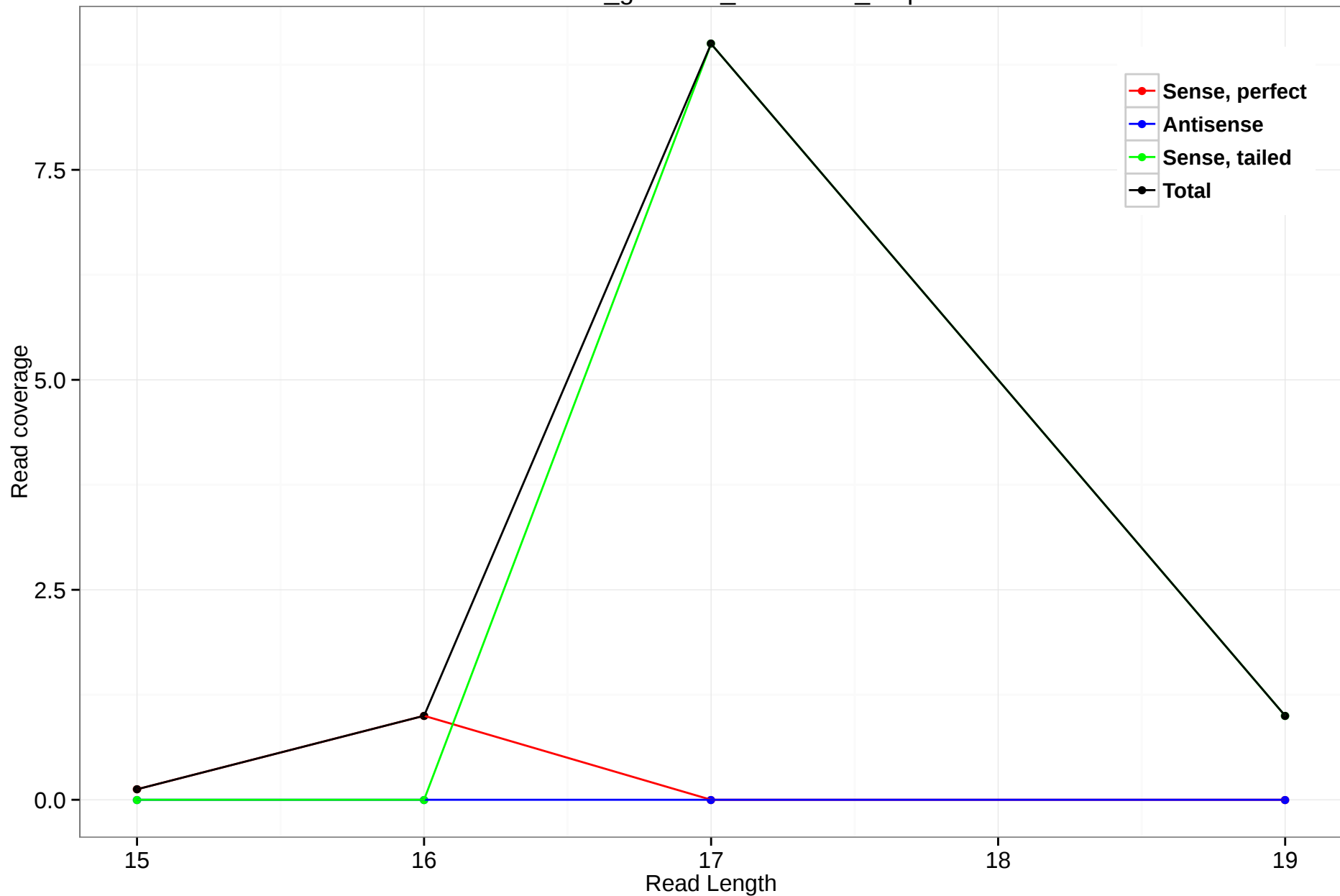
rheMac3_genscan_chr6.1321_3.5p
