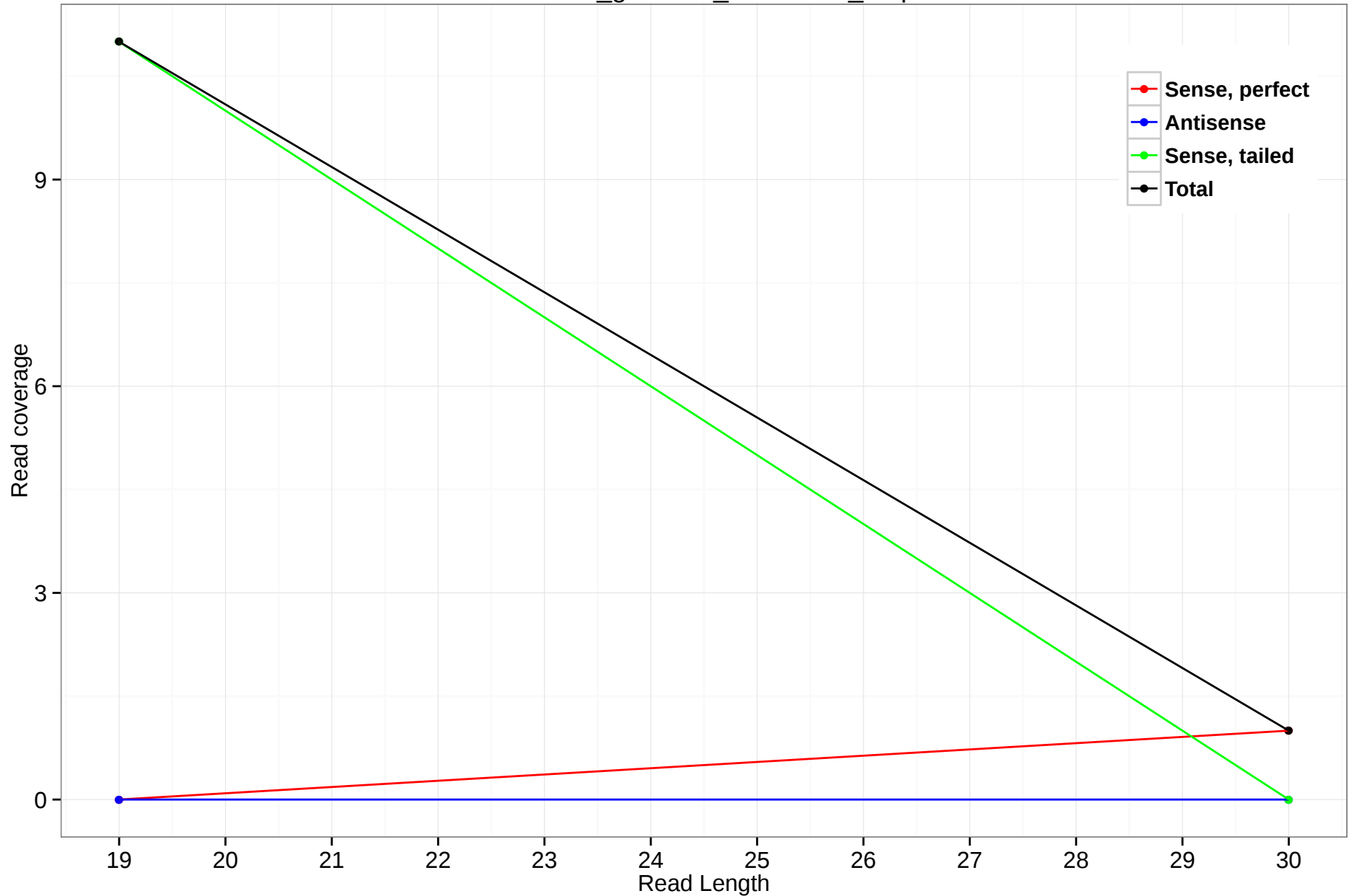
rheMac3_genscan_chr6.1306_5.5p
