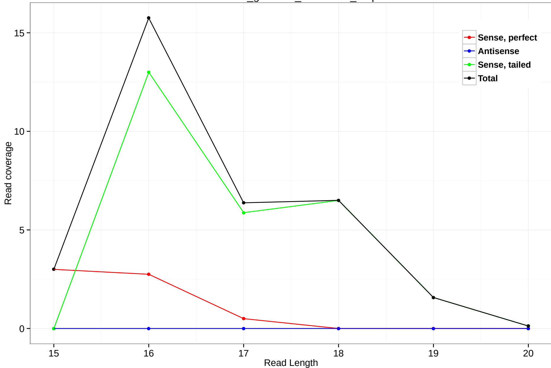
rheMac3_genscan_chr6.1294_2.3p
