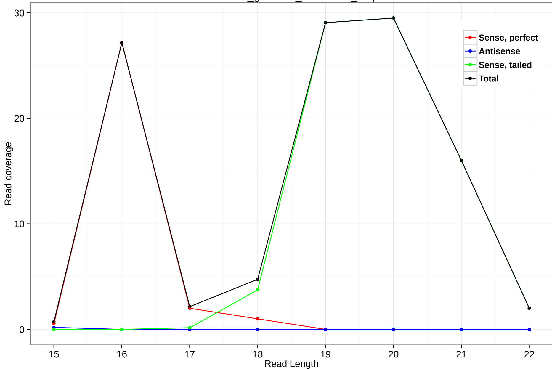
rheMac3_genscan_chr6.1266_0.5p
