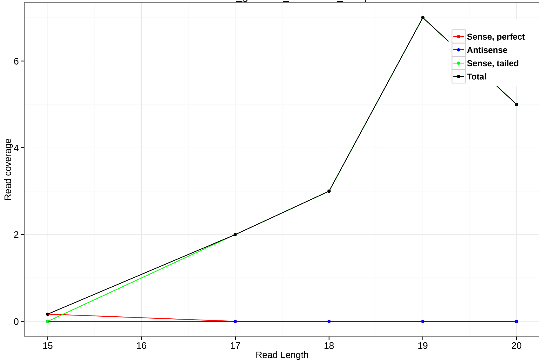
rheMac3_genscan_chr6.1088_19.5p
