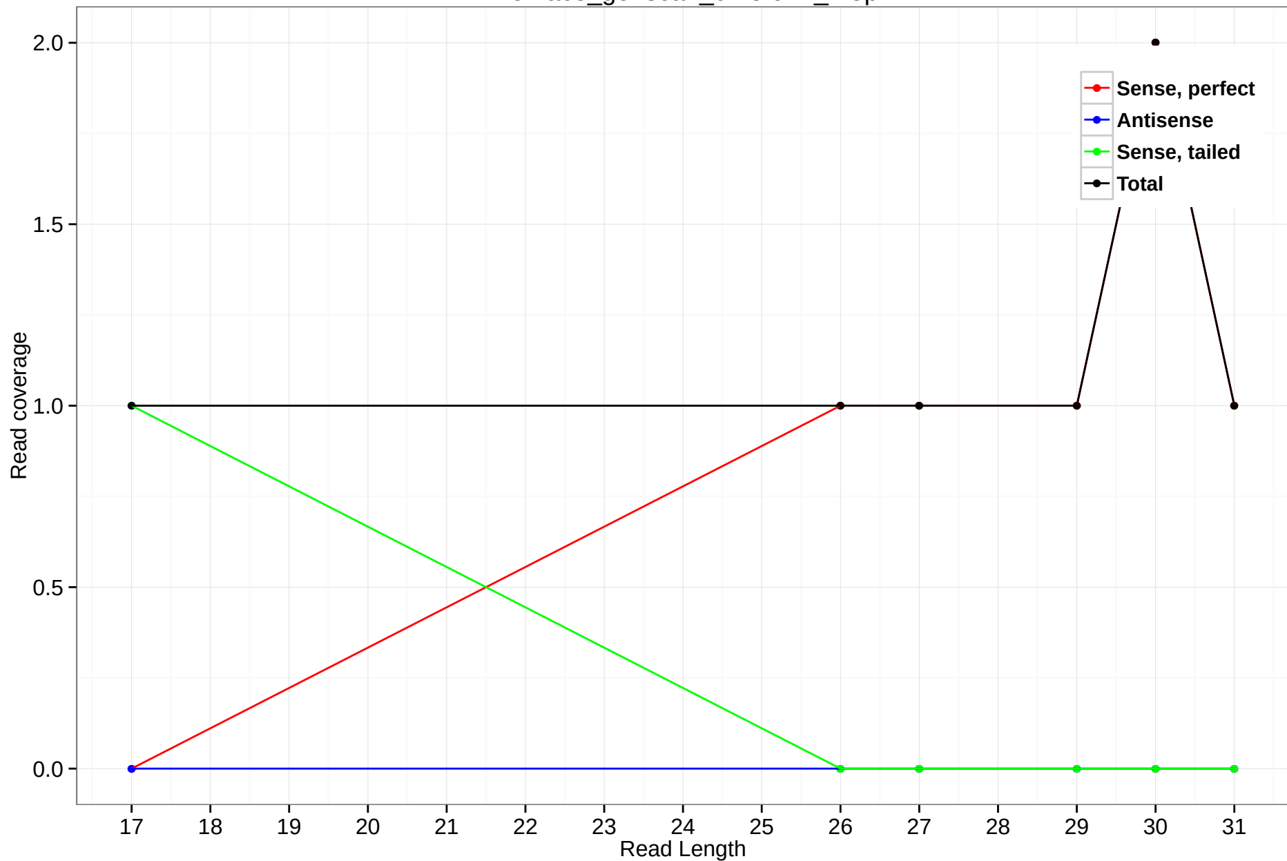
rheMac3_genscan_chr5.944_1.5p
