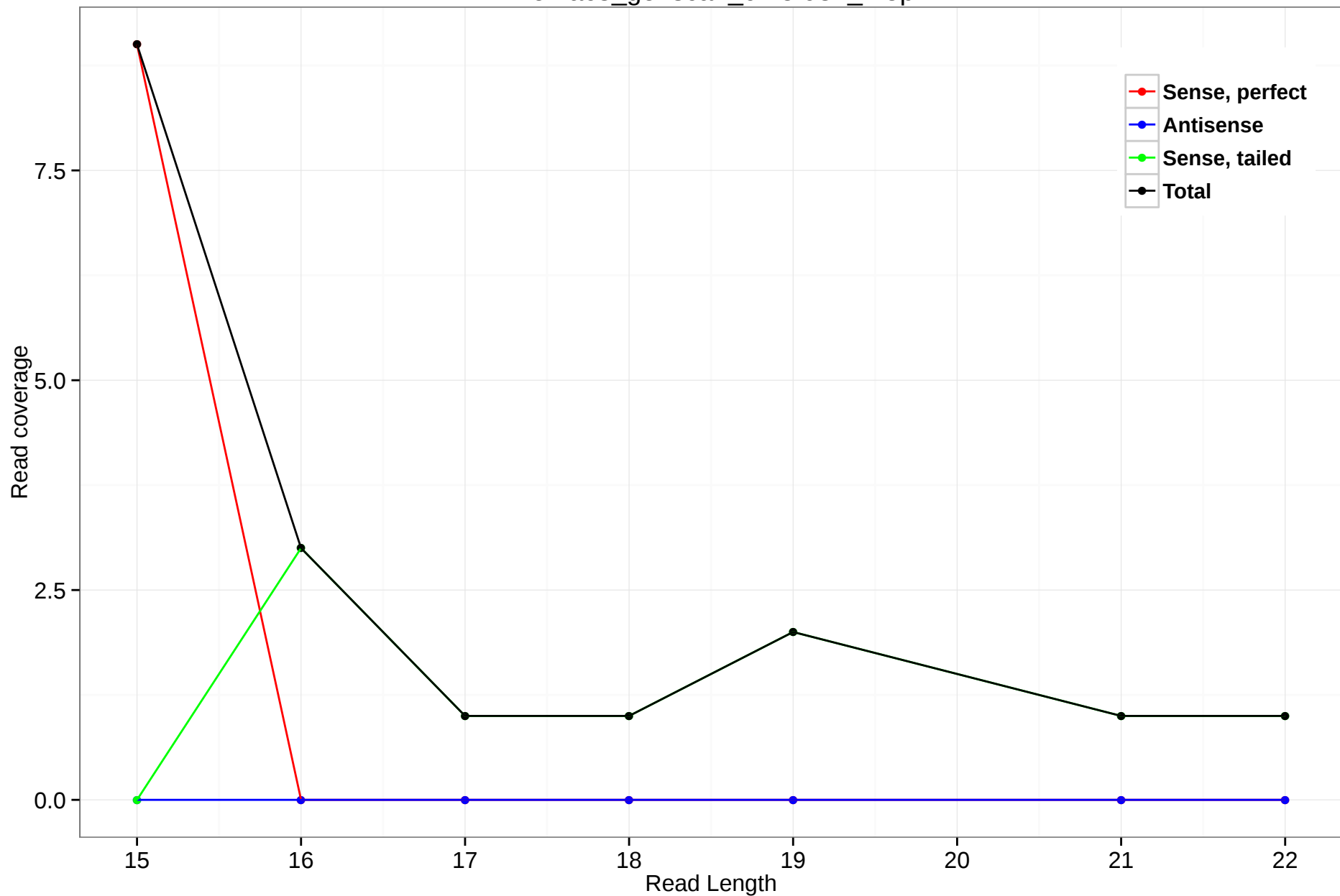
rheMac3_genscan_chr5.934_1.5p
