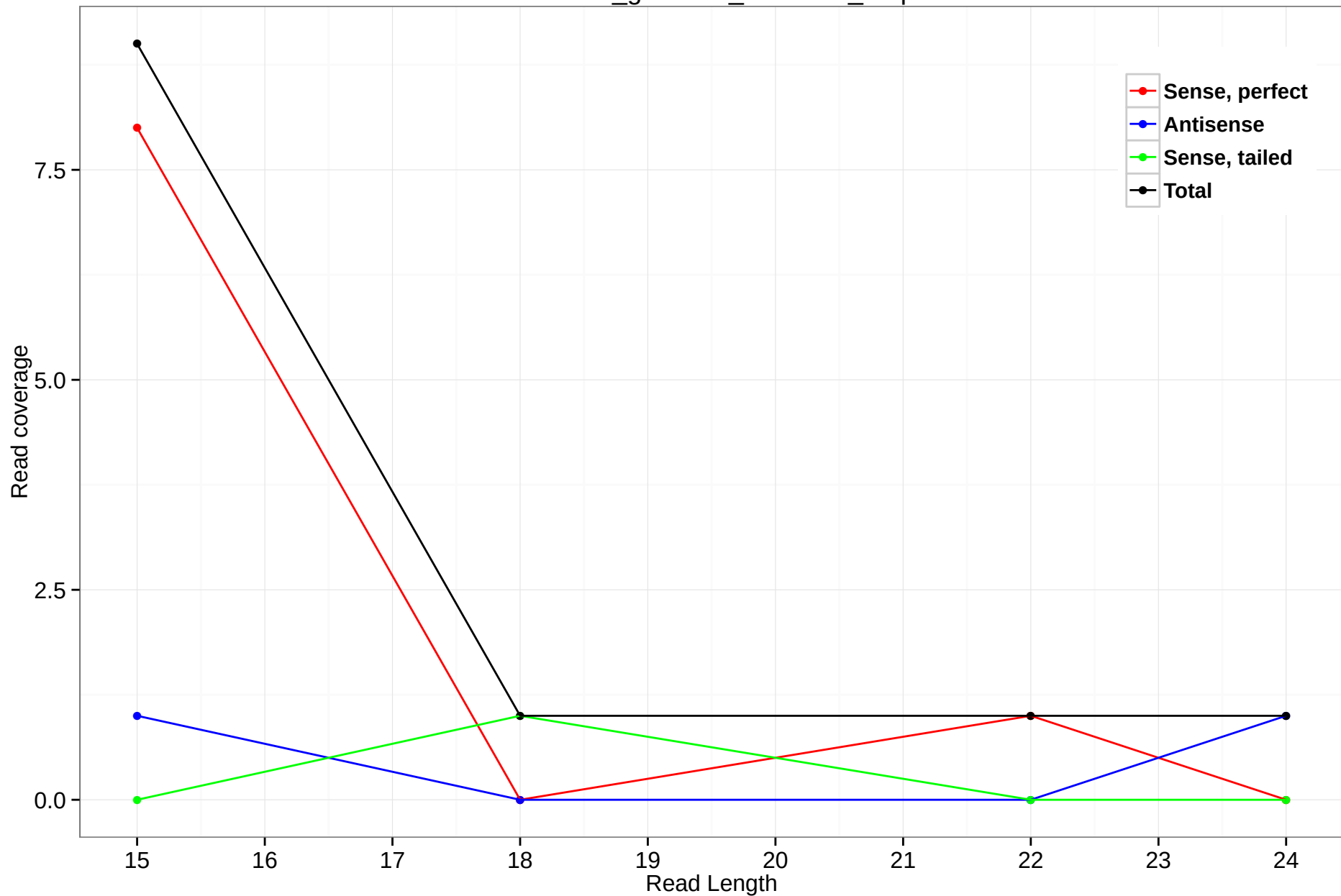
rheMac3_genscan_chr5.892_5.5p
