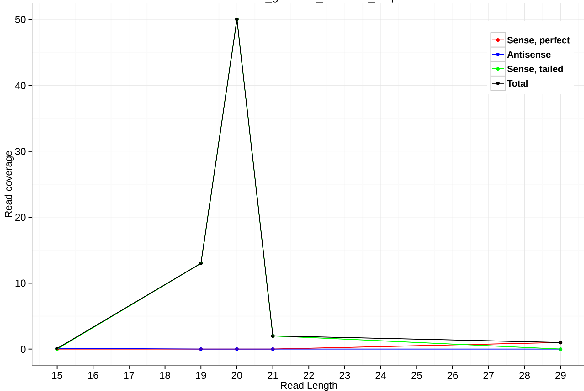
rheMac3_genscan_chr5.880_7.3p
