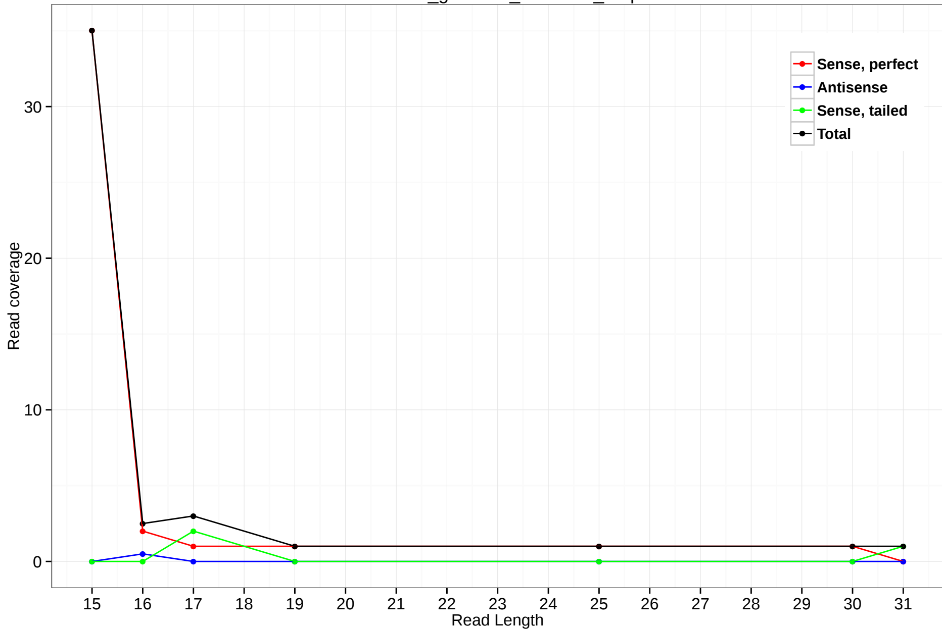
rheMac3_genscan_chr5.878_0.5p
