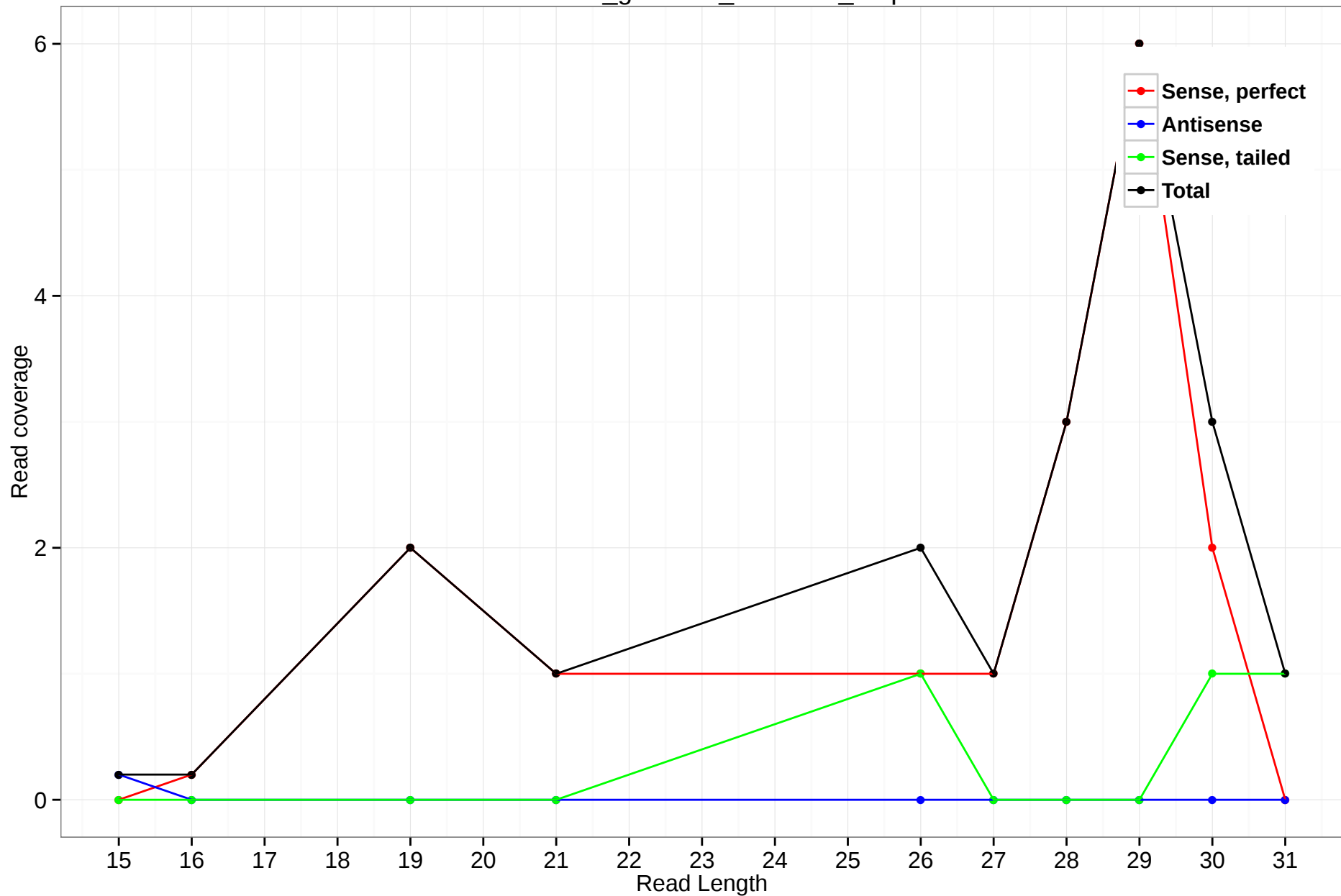
rheMac3_genscan_chr5.860_7.3p
