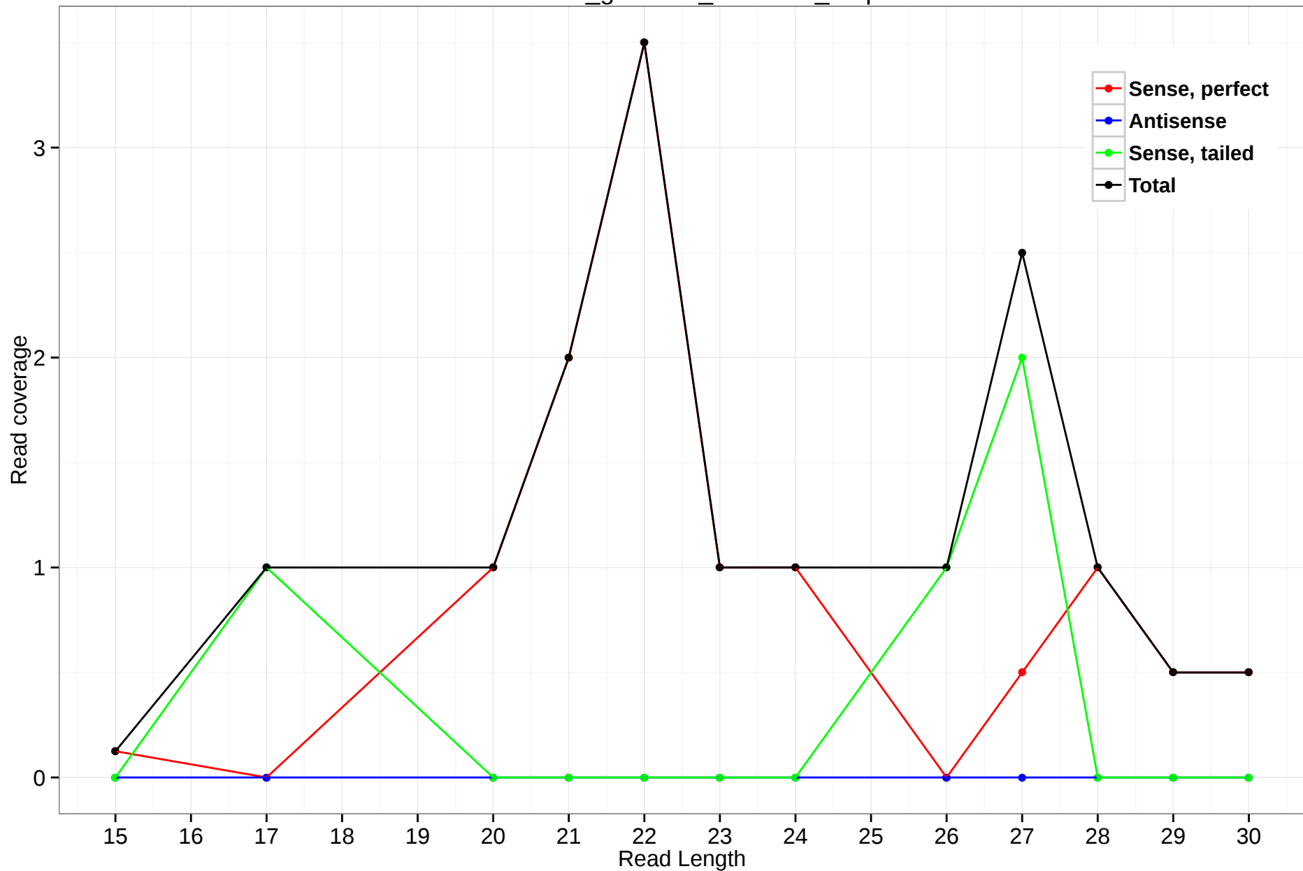
rheMac3_genscan_chr5.620_6.5p
