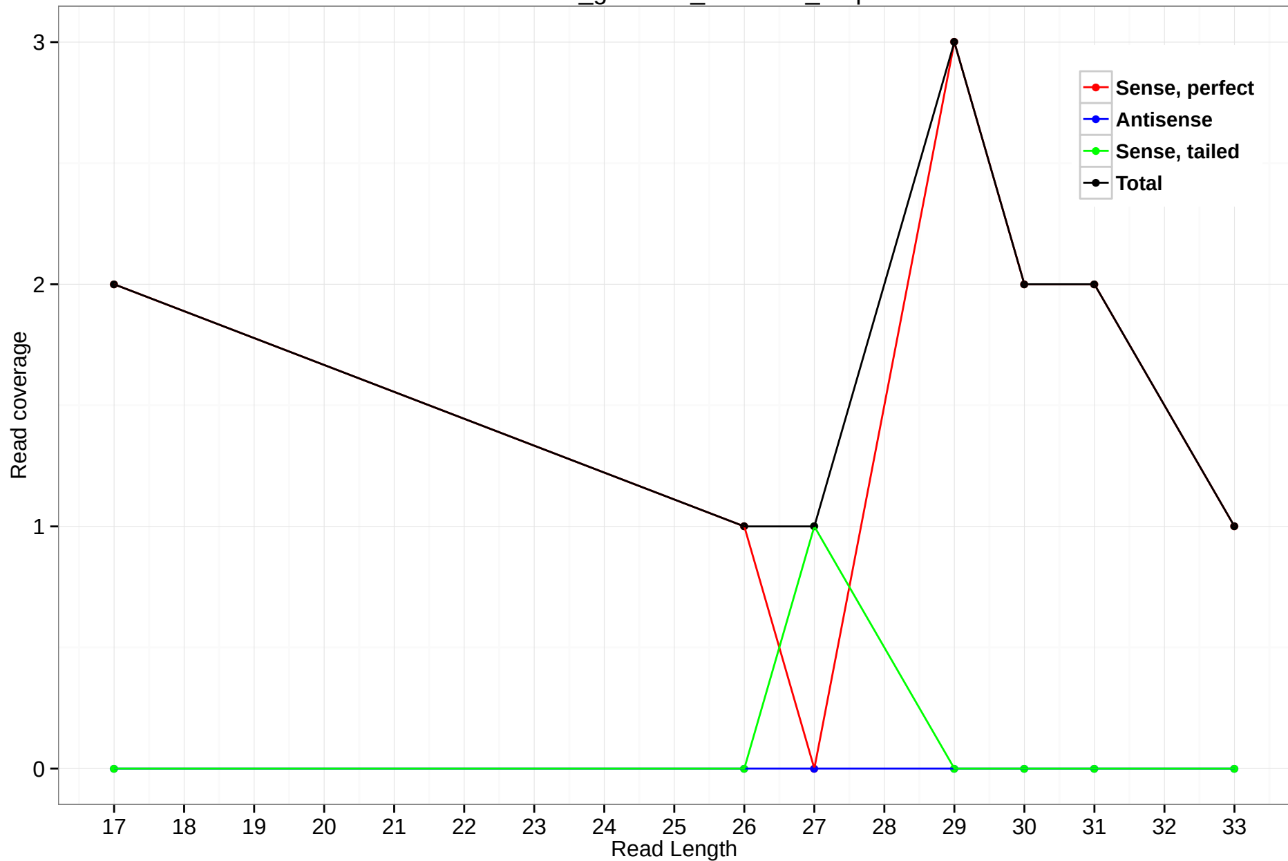
rheMac3_genscan_chr5.594_3.5p
