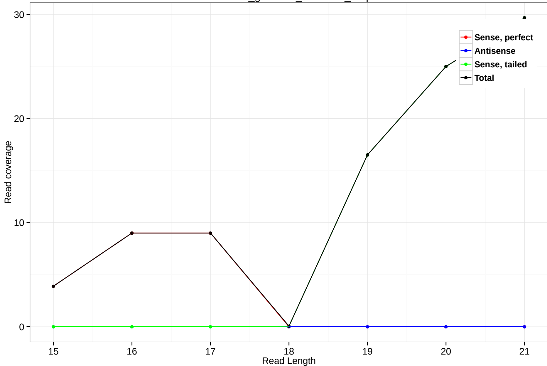
rheMac3_genscan_chr5.500_6.3p
