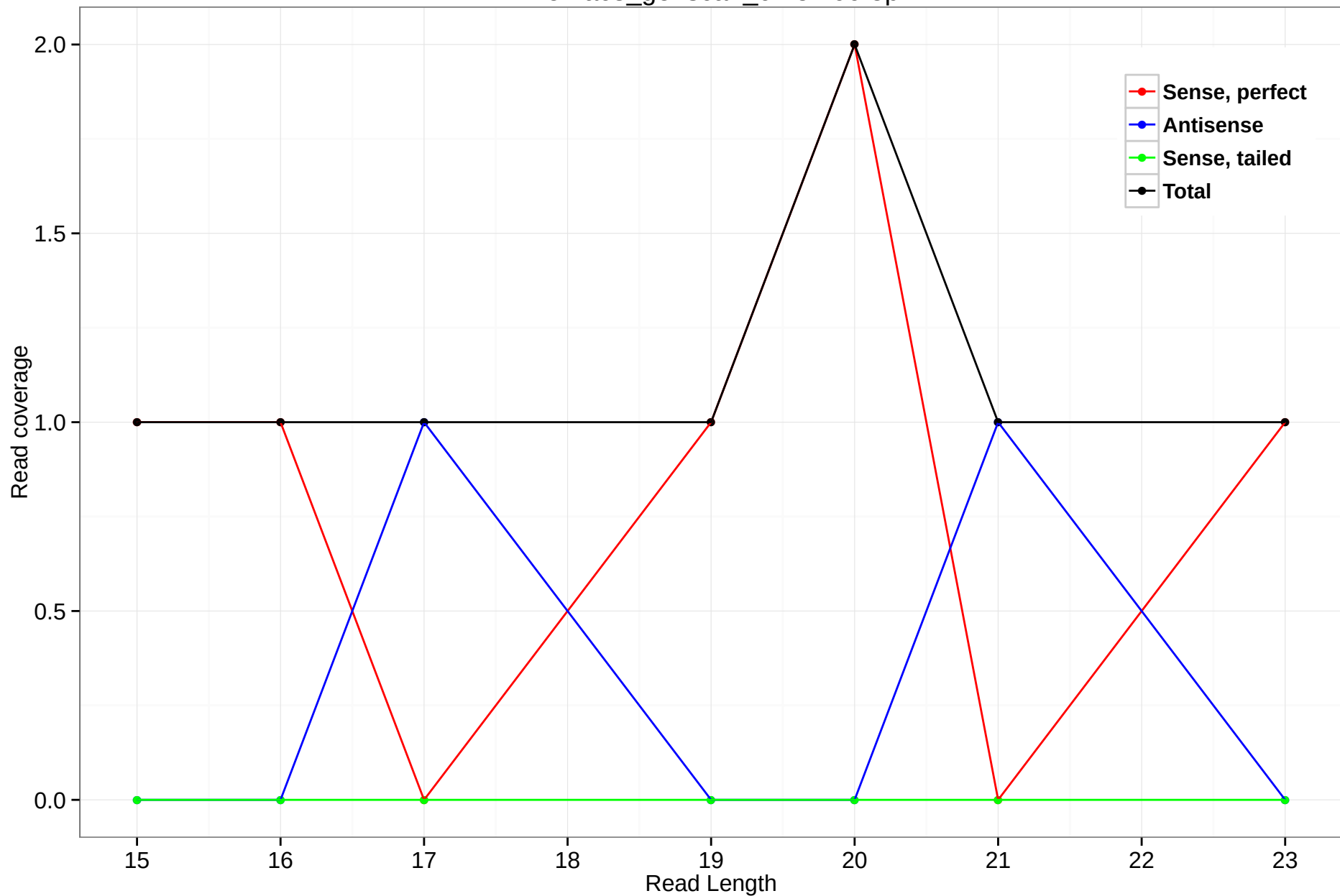
rheMac3_genscan_chr5.499.5p
