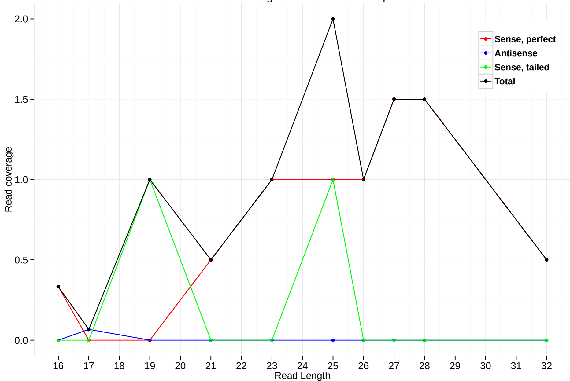
rheMac3_genscan_chr5.495_2.5p
