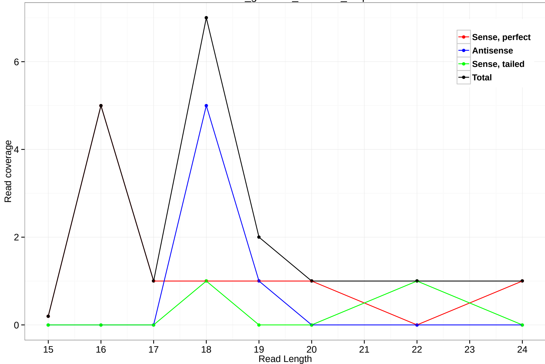
rheMac3_genscan_chr5.417_1.5p
