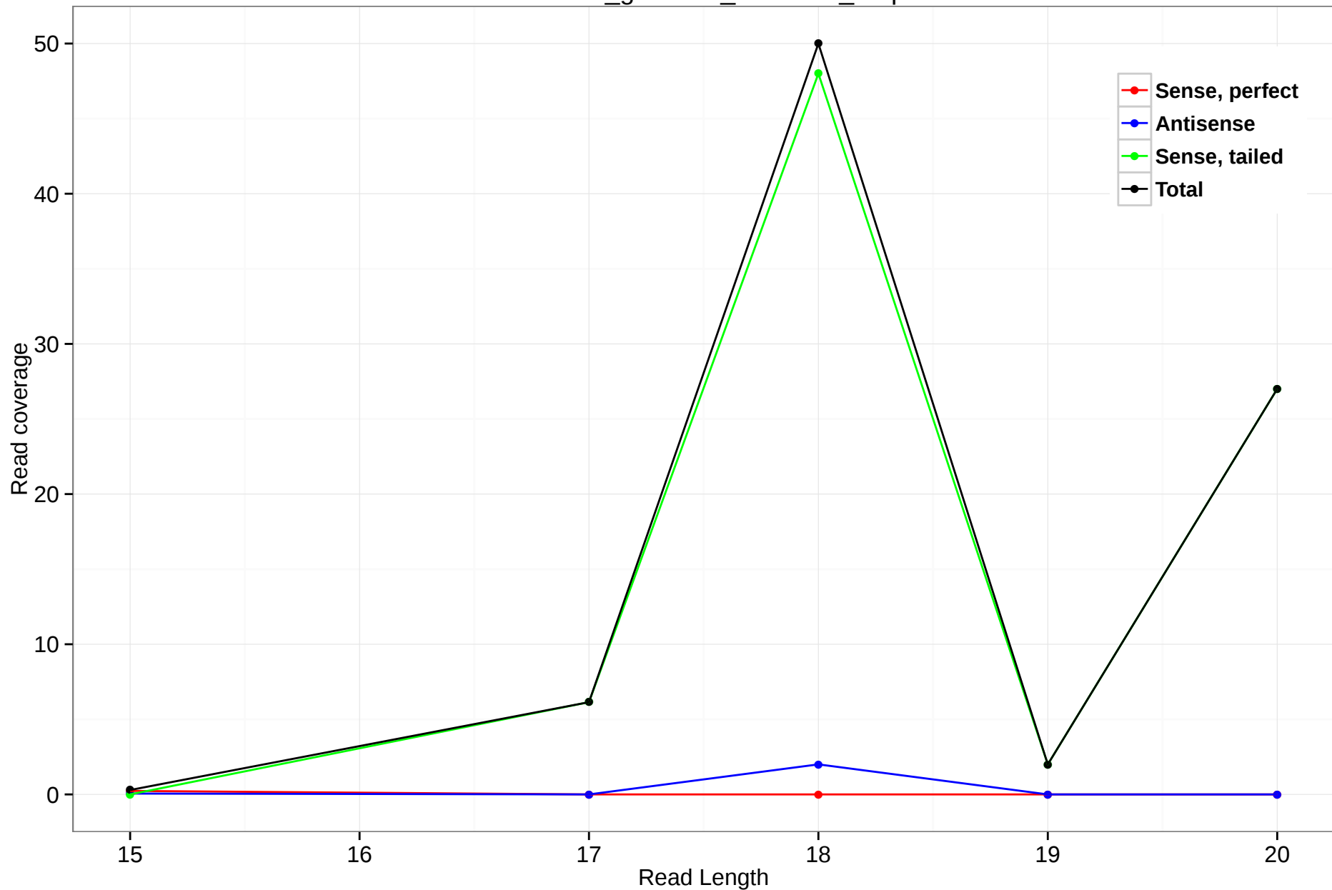
rheMac3_genscan_chr5.399_6.3p
