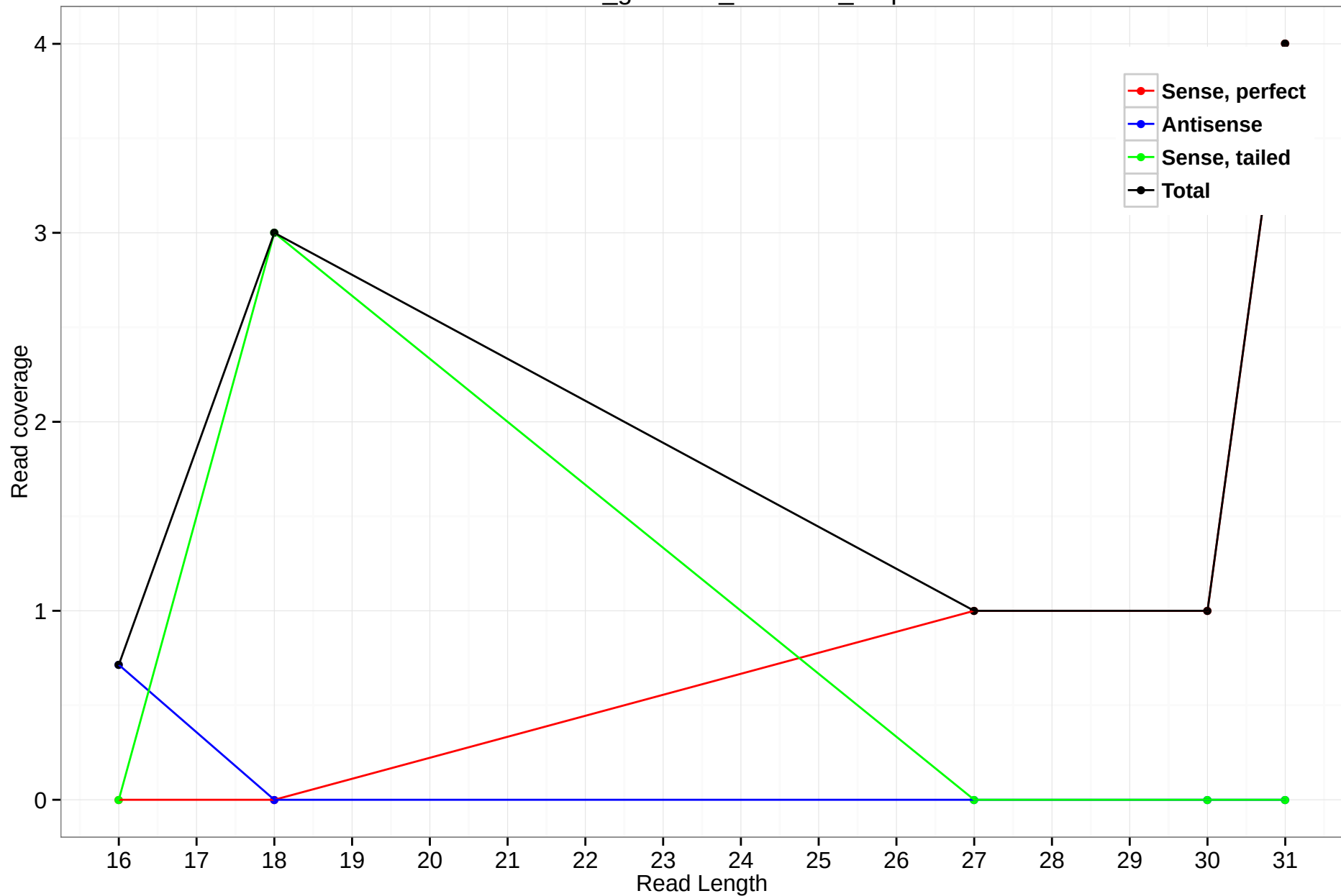
rheMac3_genscan_chr5.391_7.5p
