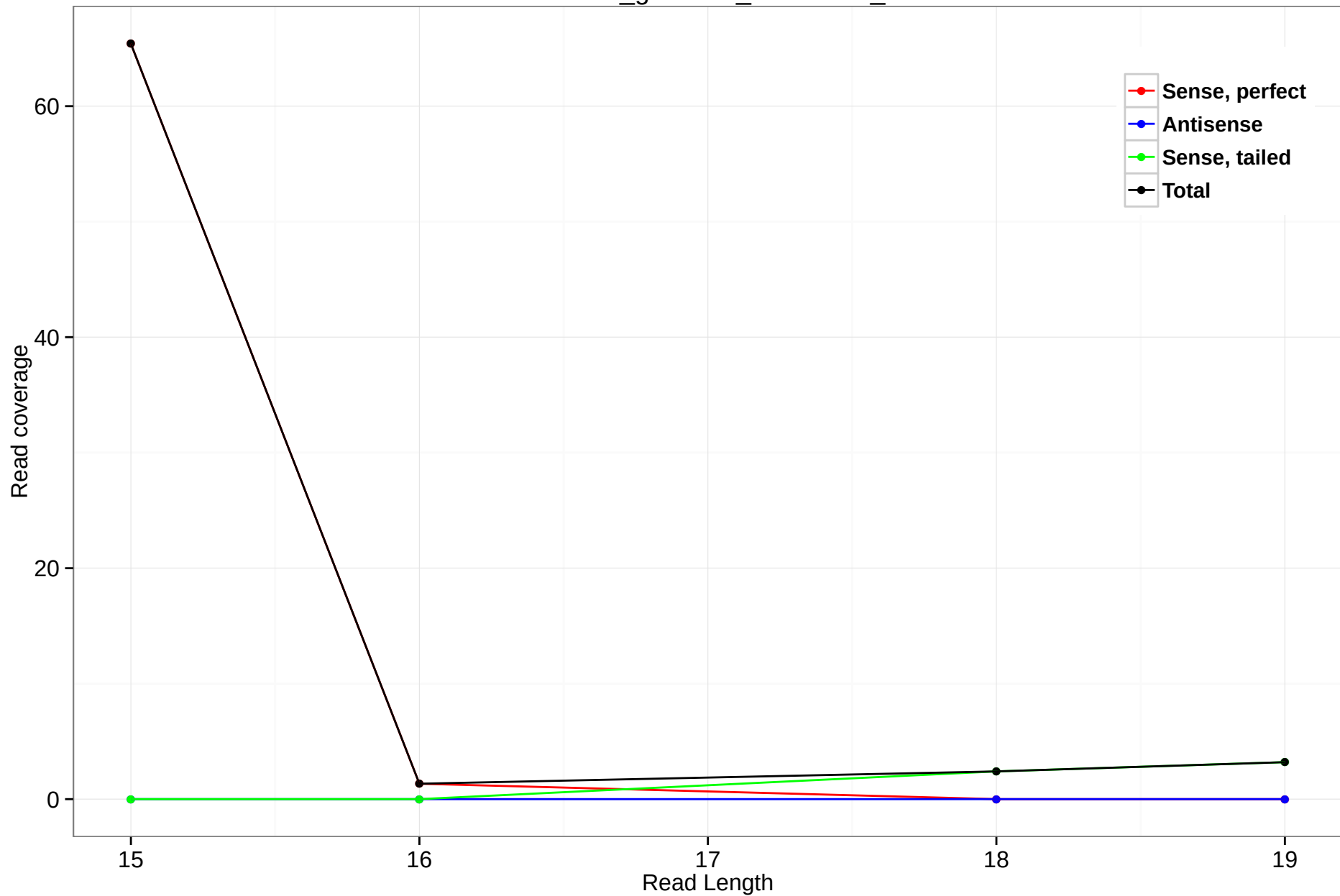
rheMac3_genscan_chr5.2809_0
