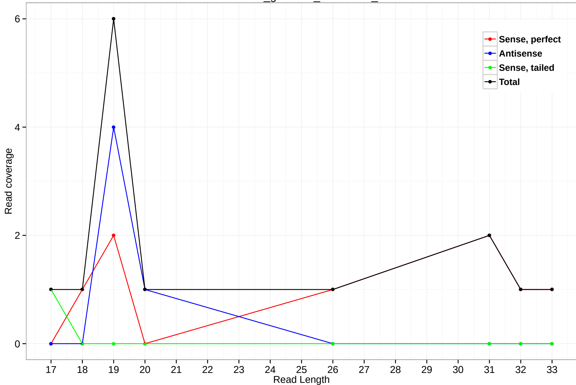
rheMac3_genscan_chr5.2650_1
