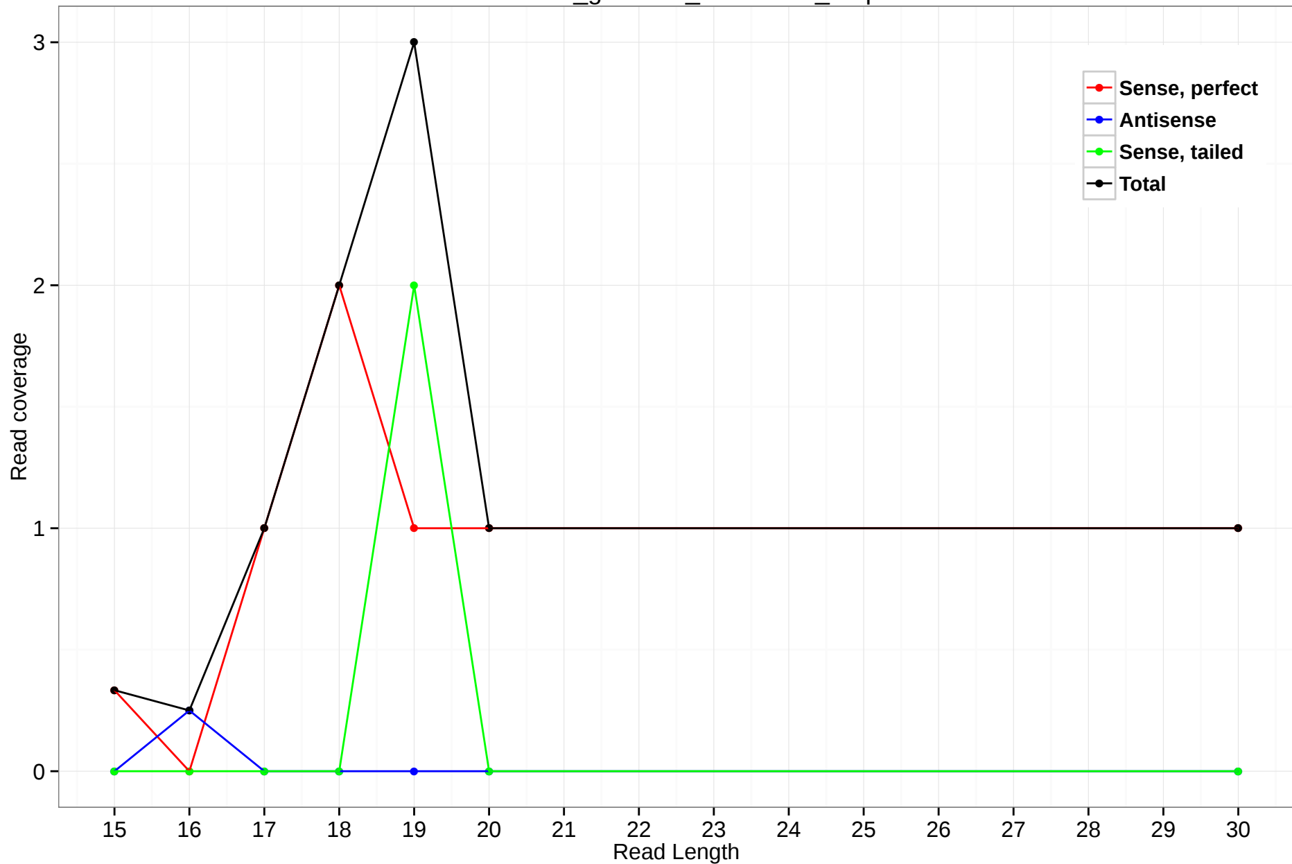
rheMac3_genscan_chr5.2598_1.3p
