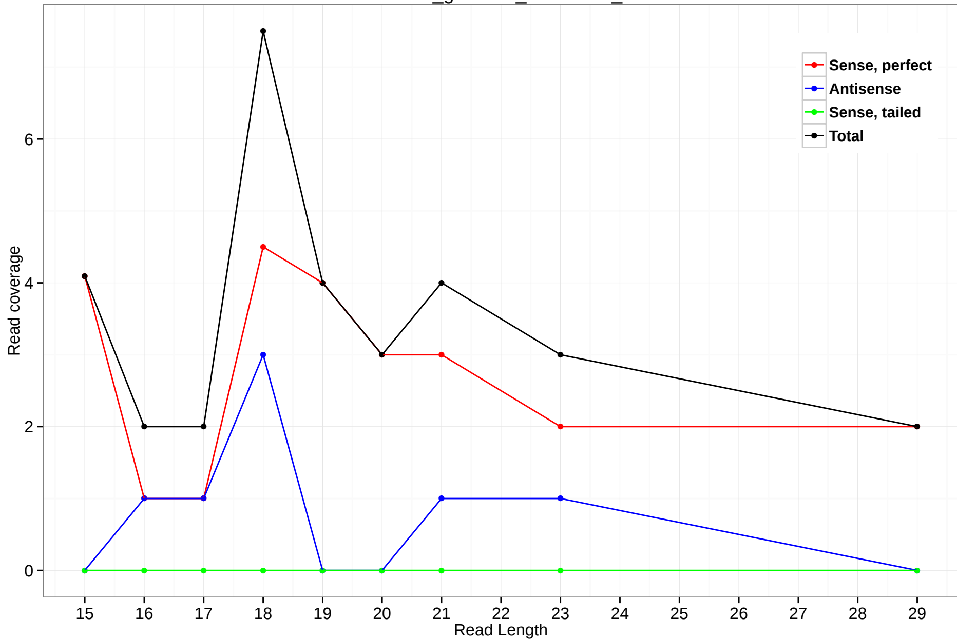
rheMac3_genscan_chr5.2596_11
