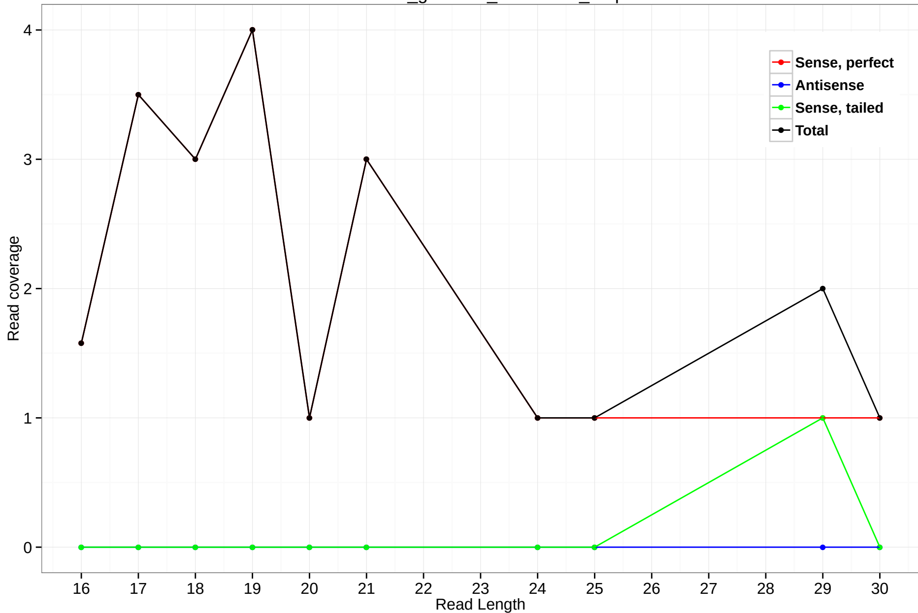
rheMac3_genscan_chr5.2344_3.5p
