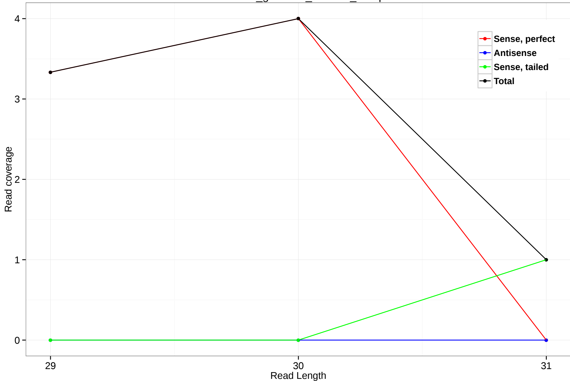
rheMac3_genscan_chr5.20_18.3p
