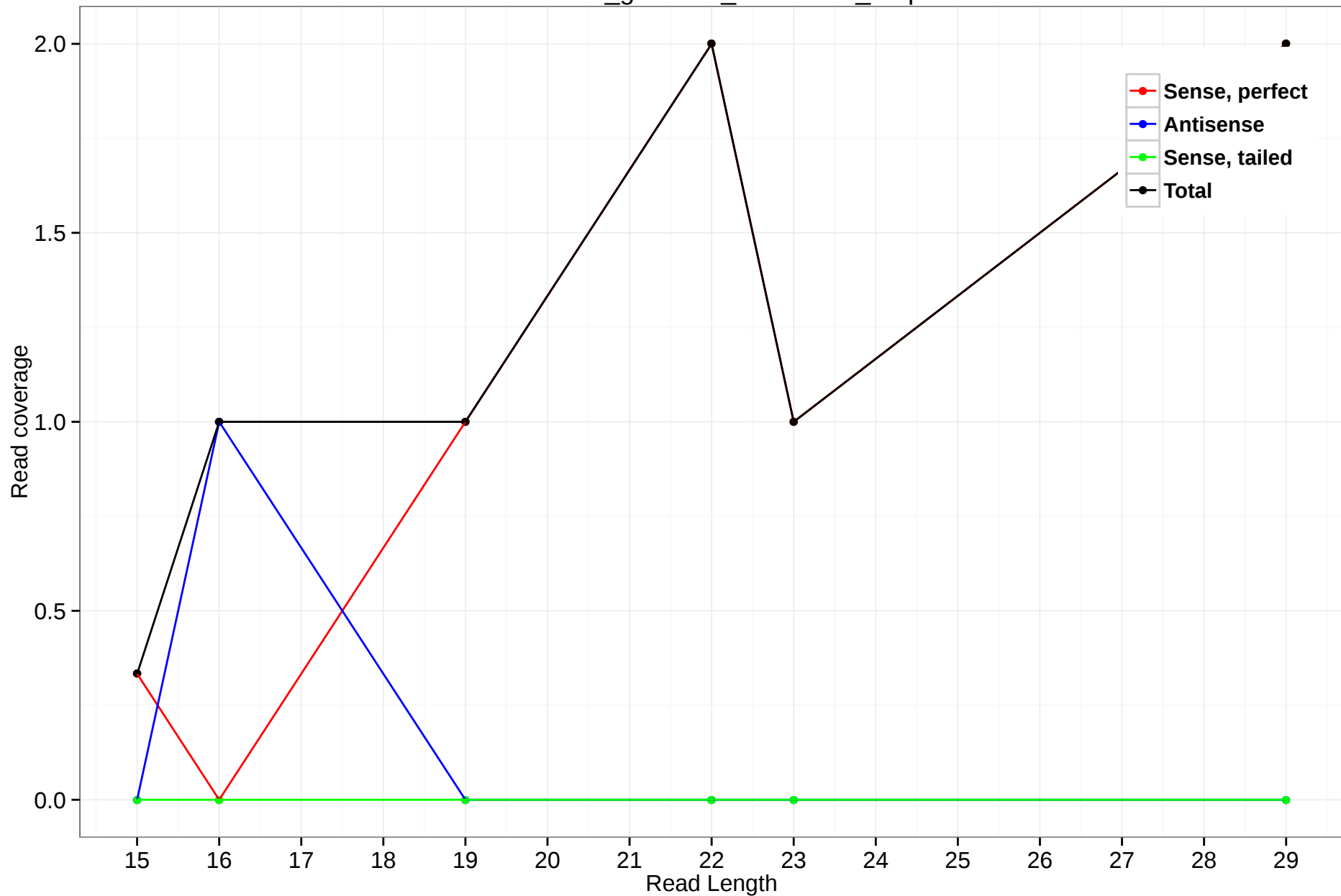
rheMac3_genscan_chr5.2096_8.5p
