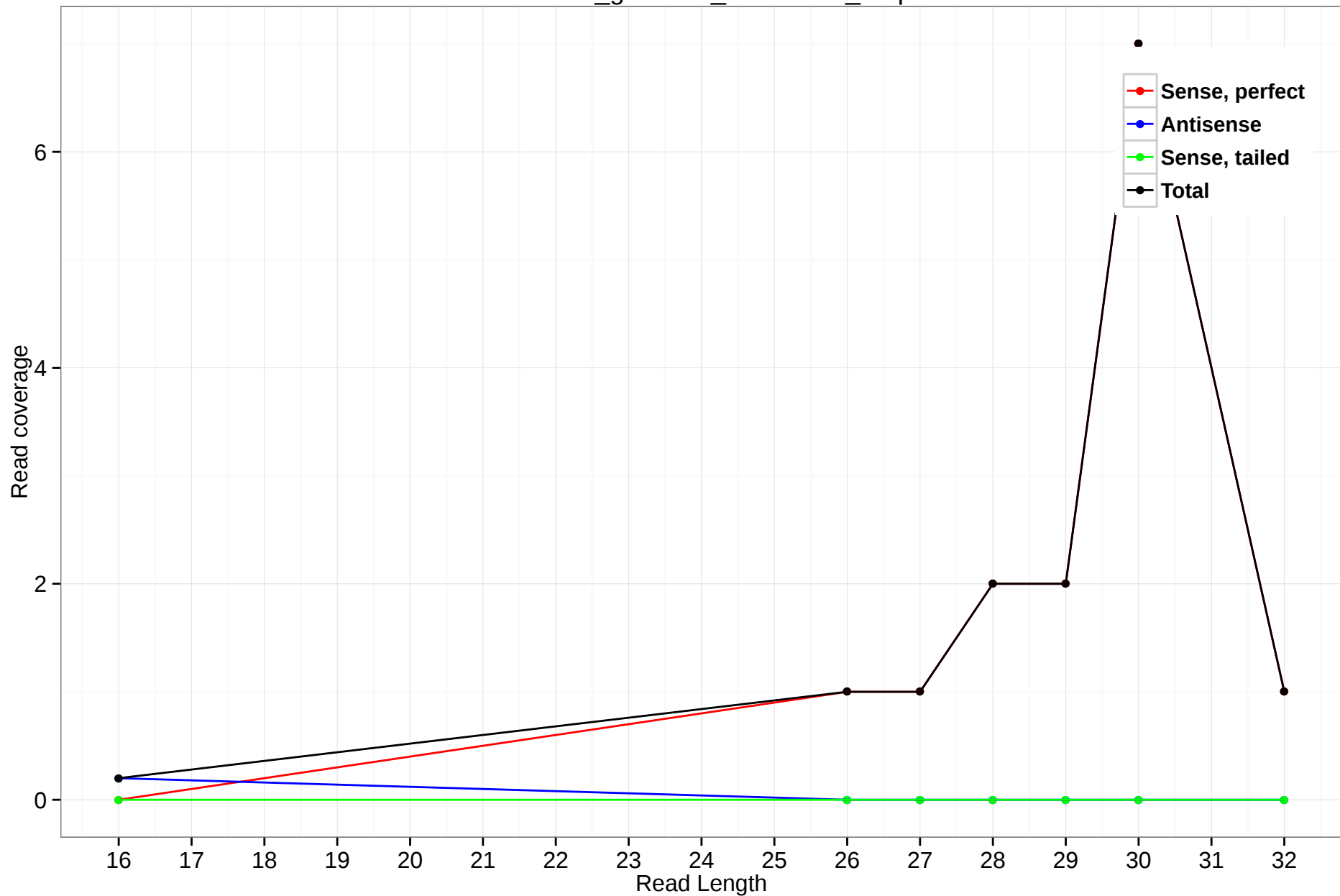
rheMac3_genscan_chr5.2092_8.3p
