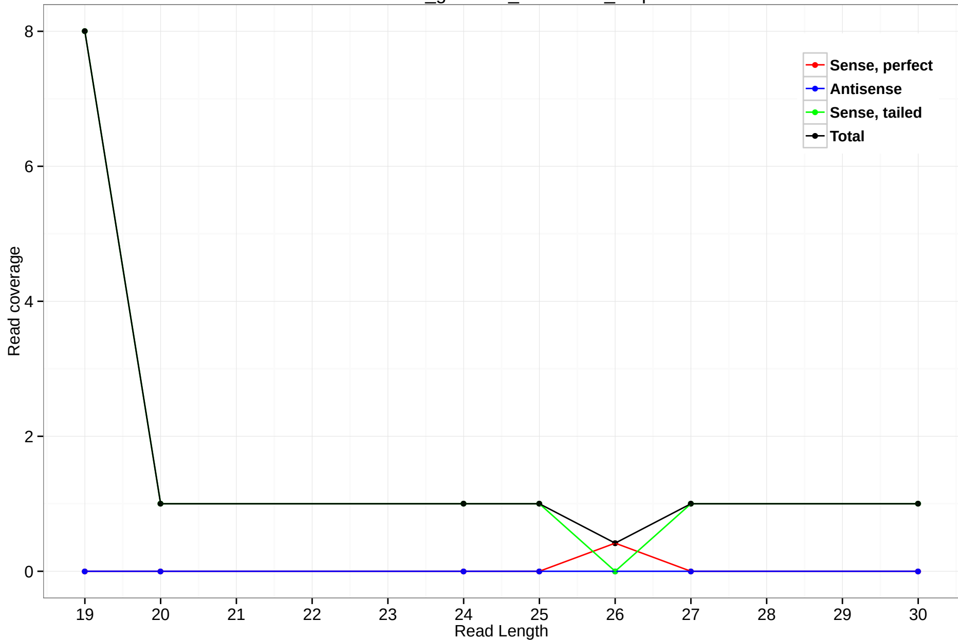
rheMac3_genscan_chr5.2054_5.3p
