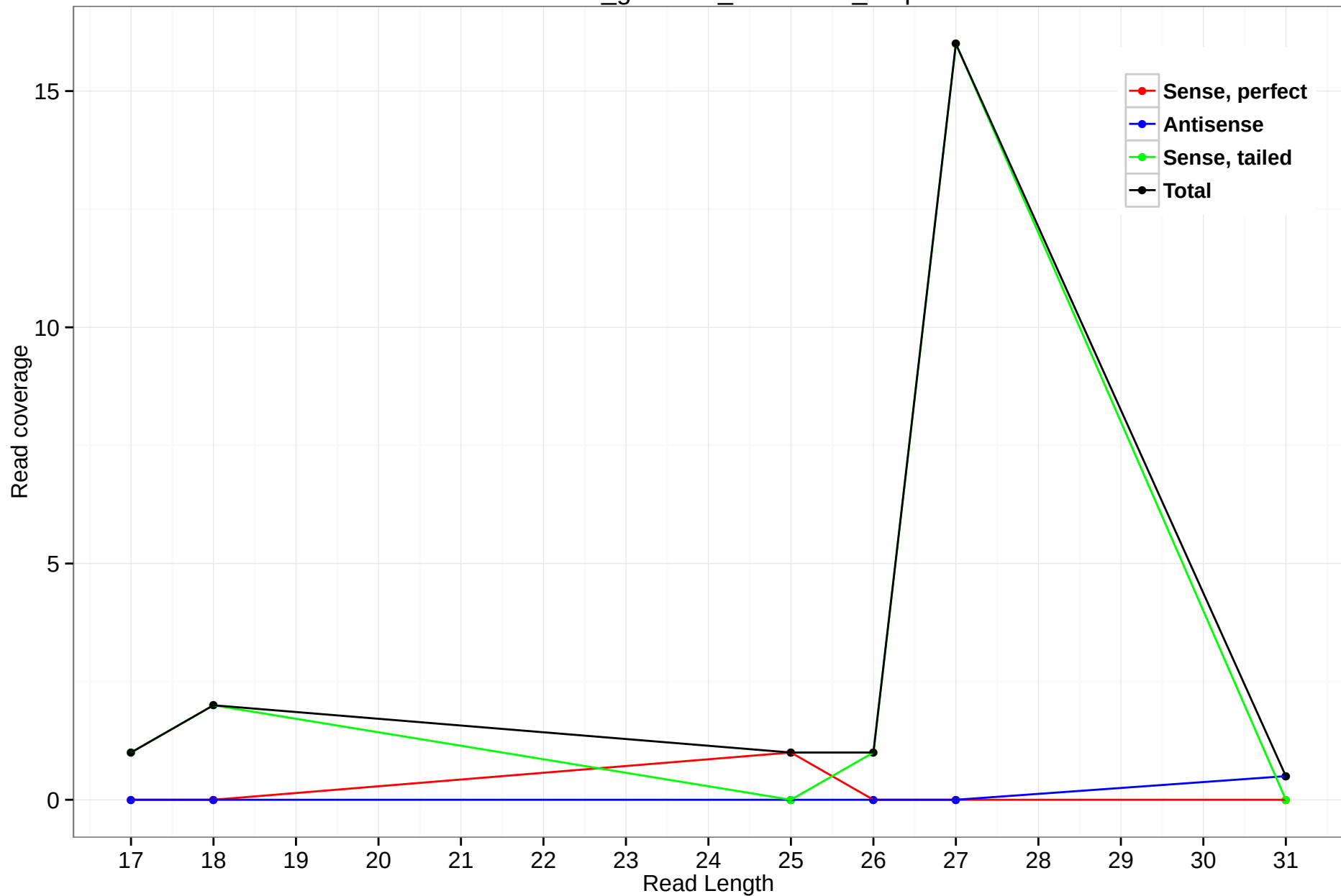
rheMac3_genscan_chr5.2005_0.5p
