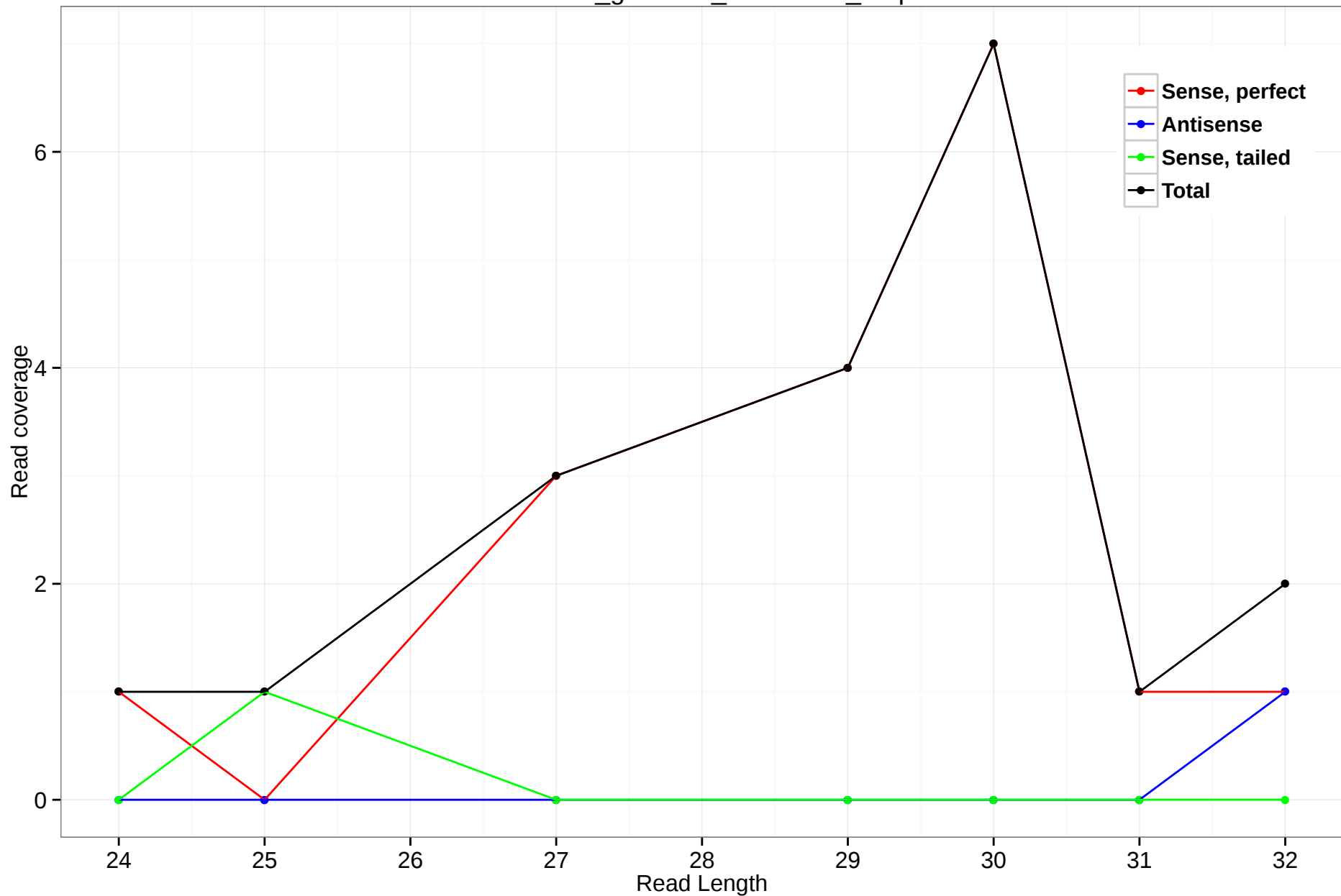
rheMac3_genscan_chr5.1921_4.5p
