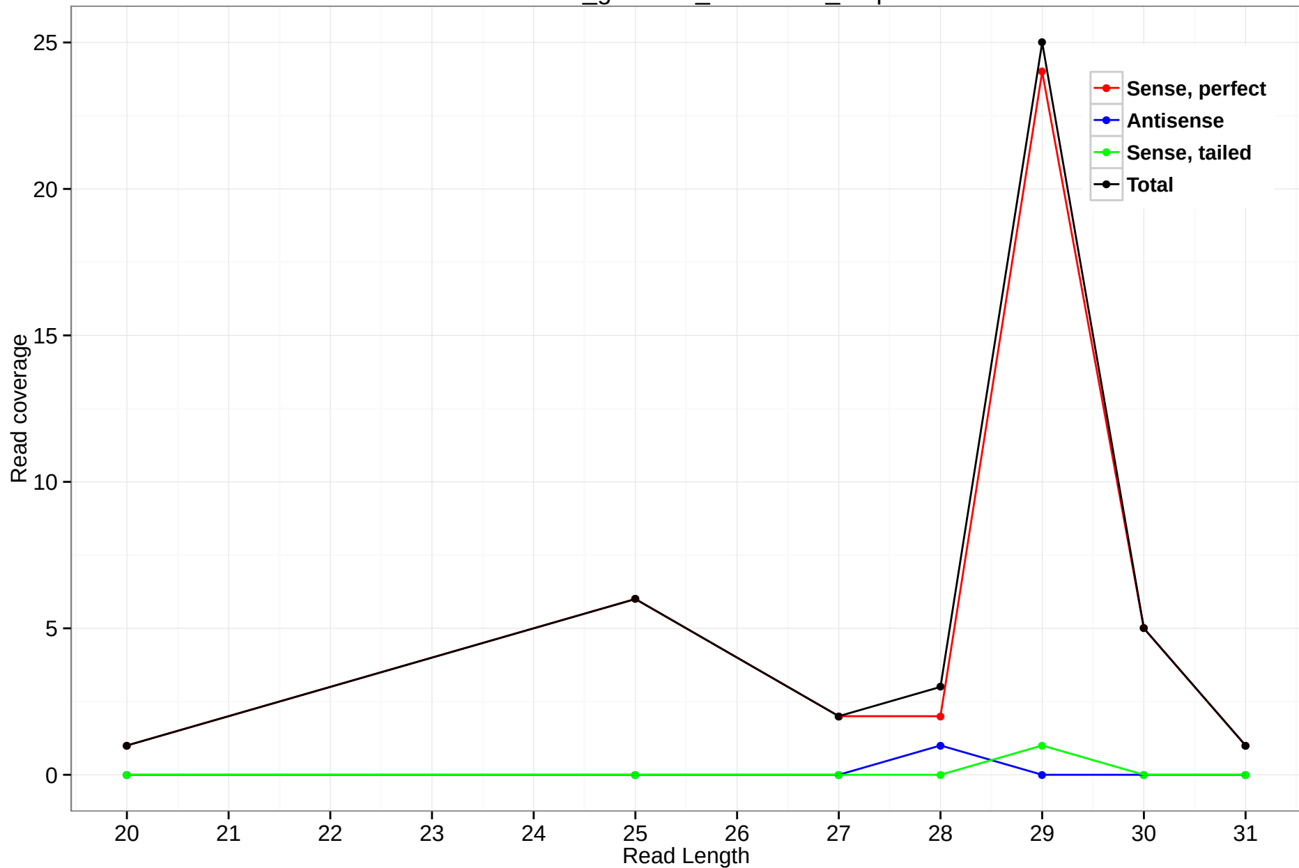
rheMac3_genscan_chr5.1921_4.3p
