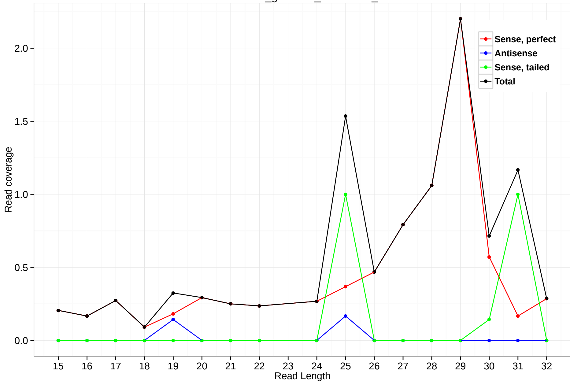
rheMac3_genscan_chr5.1872_1
