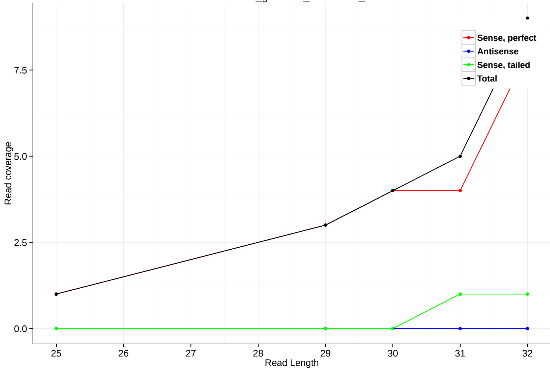
rheMac3_genscan_chr5.1821_2
