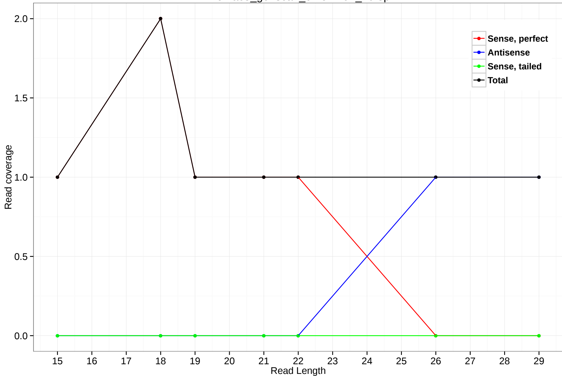
rheMac3_genscan_chr5.1791_20.3p
