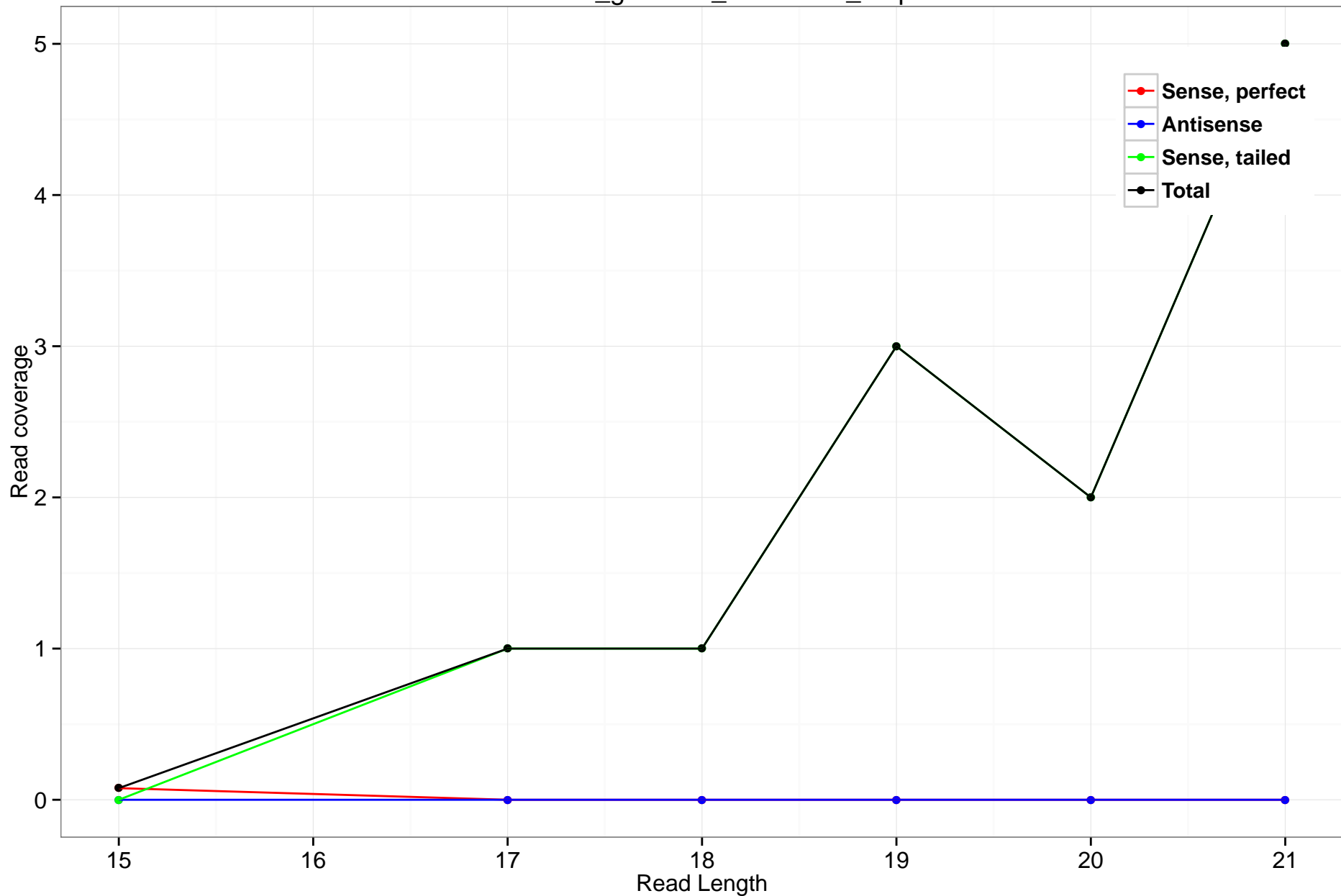
rheMac3_genscan_chr5.1758_6.5p
