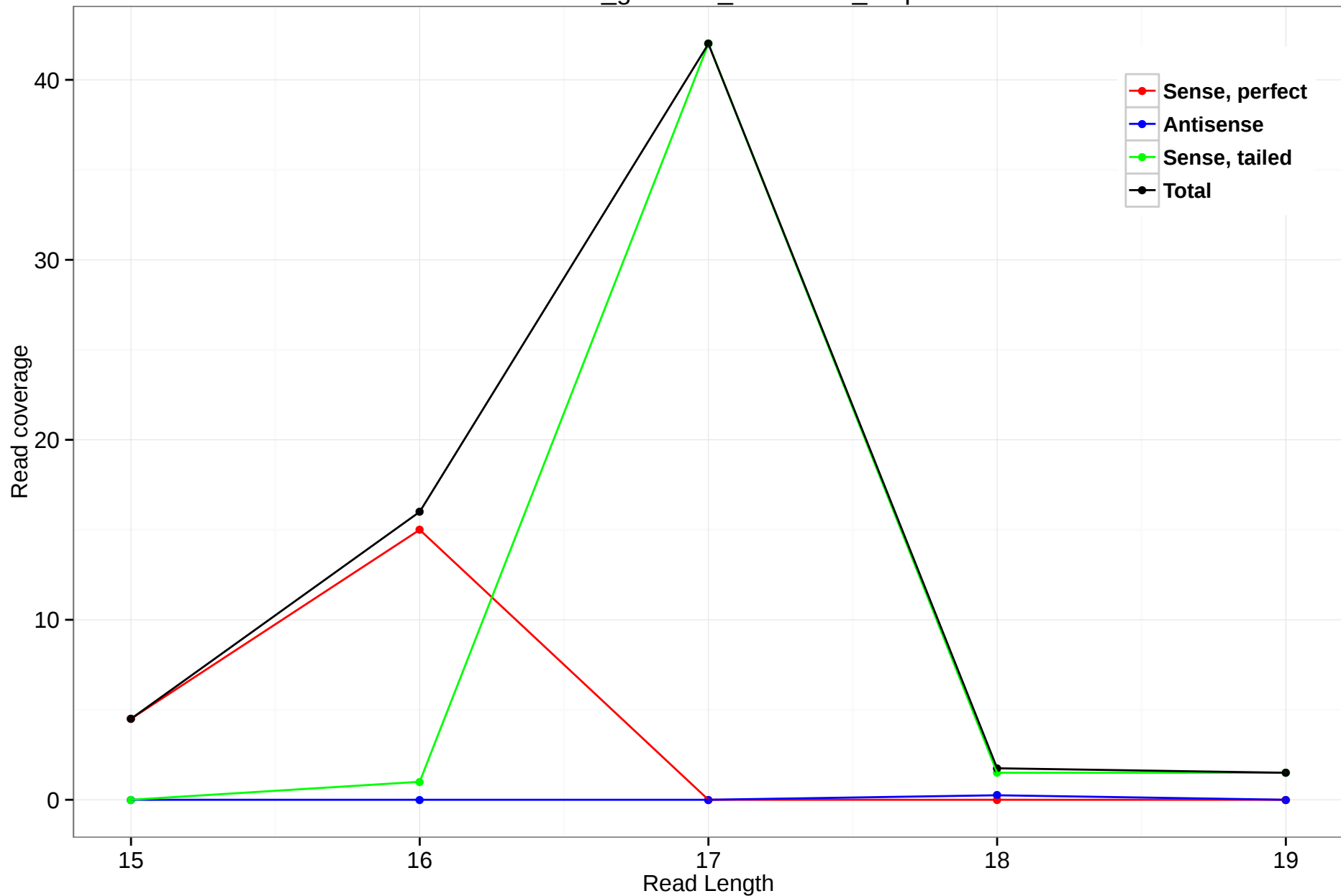
rheMac3_genscan_chr5.1681_3.3p
