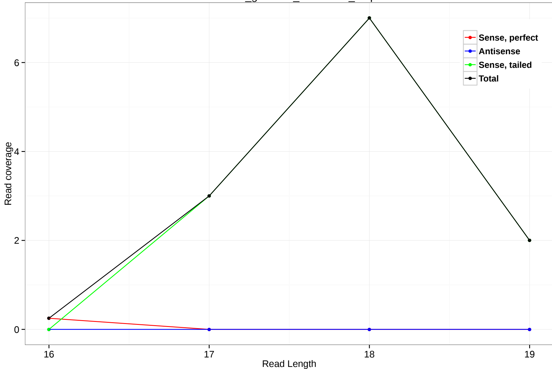
rheMac3_genscan_chr5.1670_9.5p
