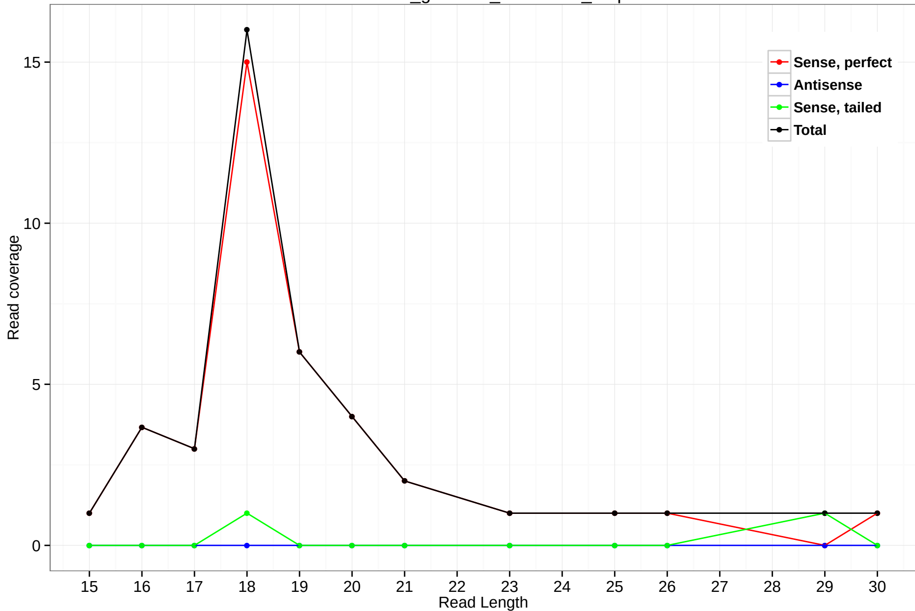
rheMac3_genscan_chr5.1669_6.5p
