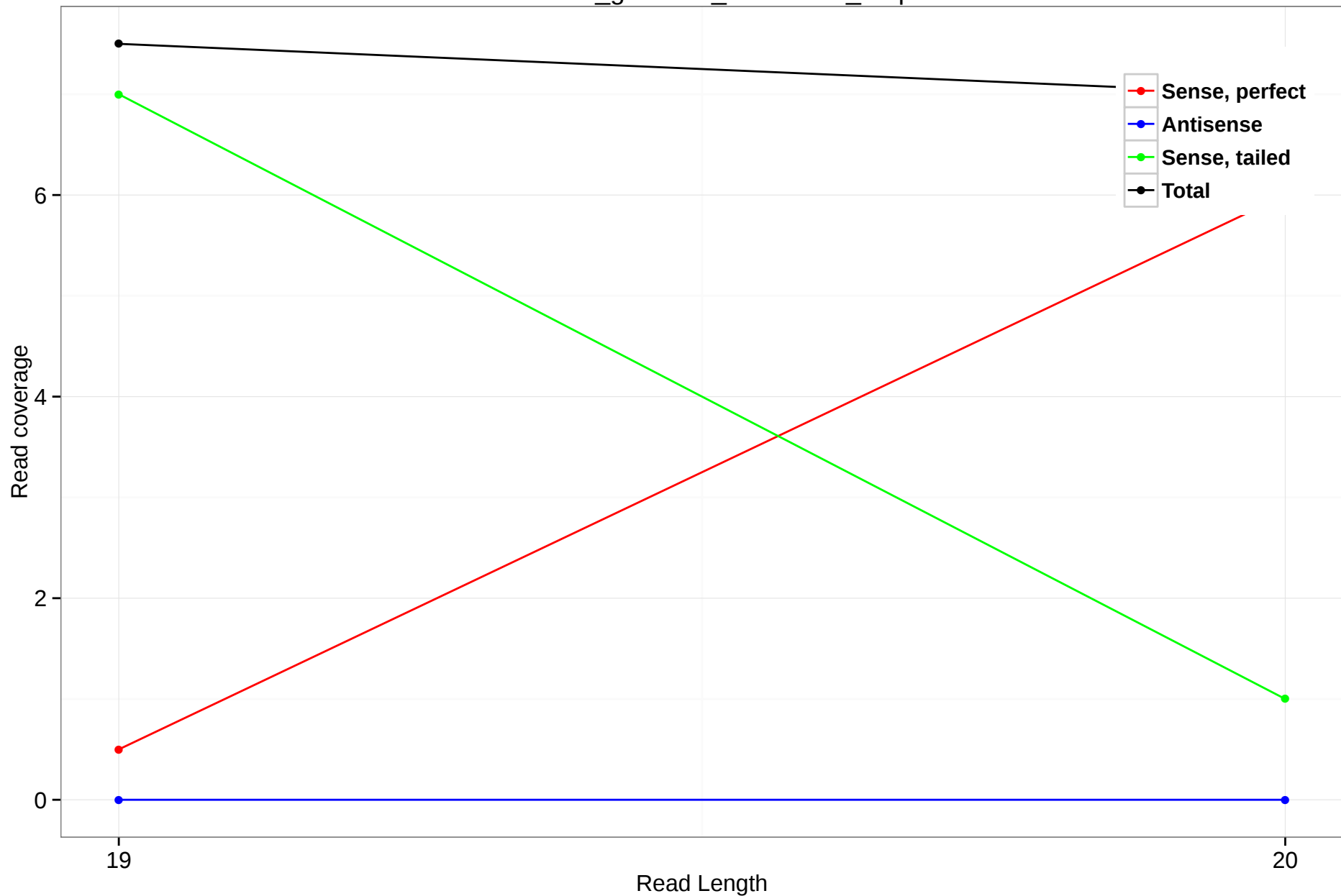
rheMac3_genscan_chr5.1566_3.3p
