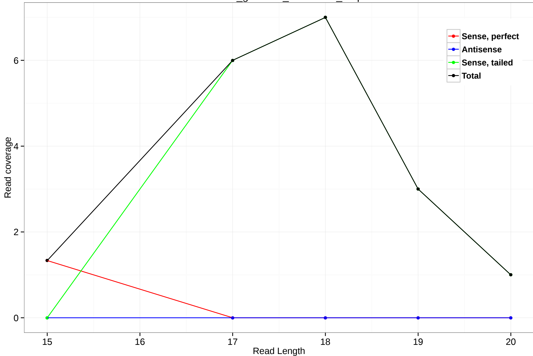
rheMac3_genscan_chr5.1548_2.3p
