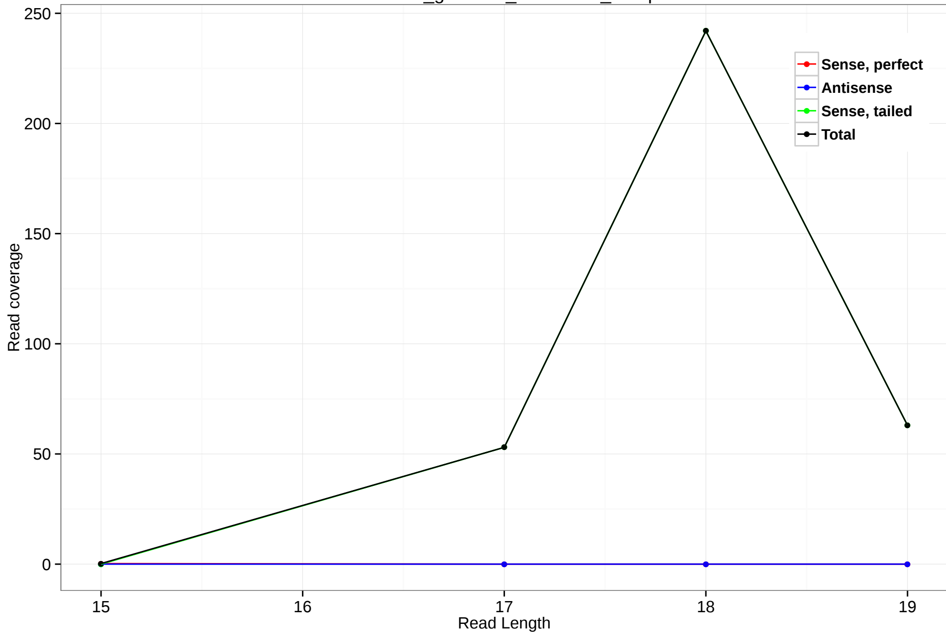
rheMac3_genscan_chr5.1448_13.5p
