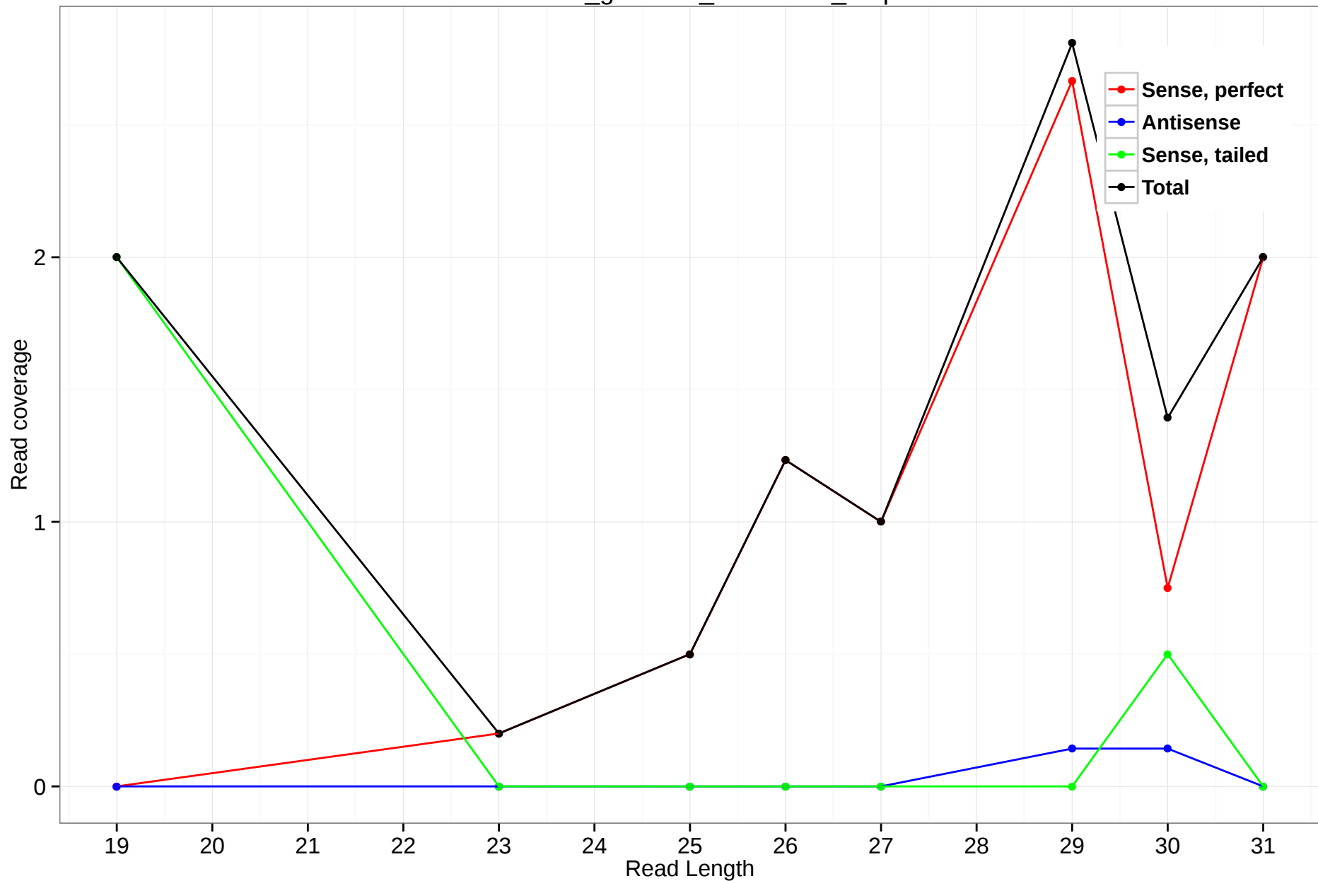
rheMac3_genscan_chr5.1311_5.3p
