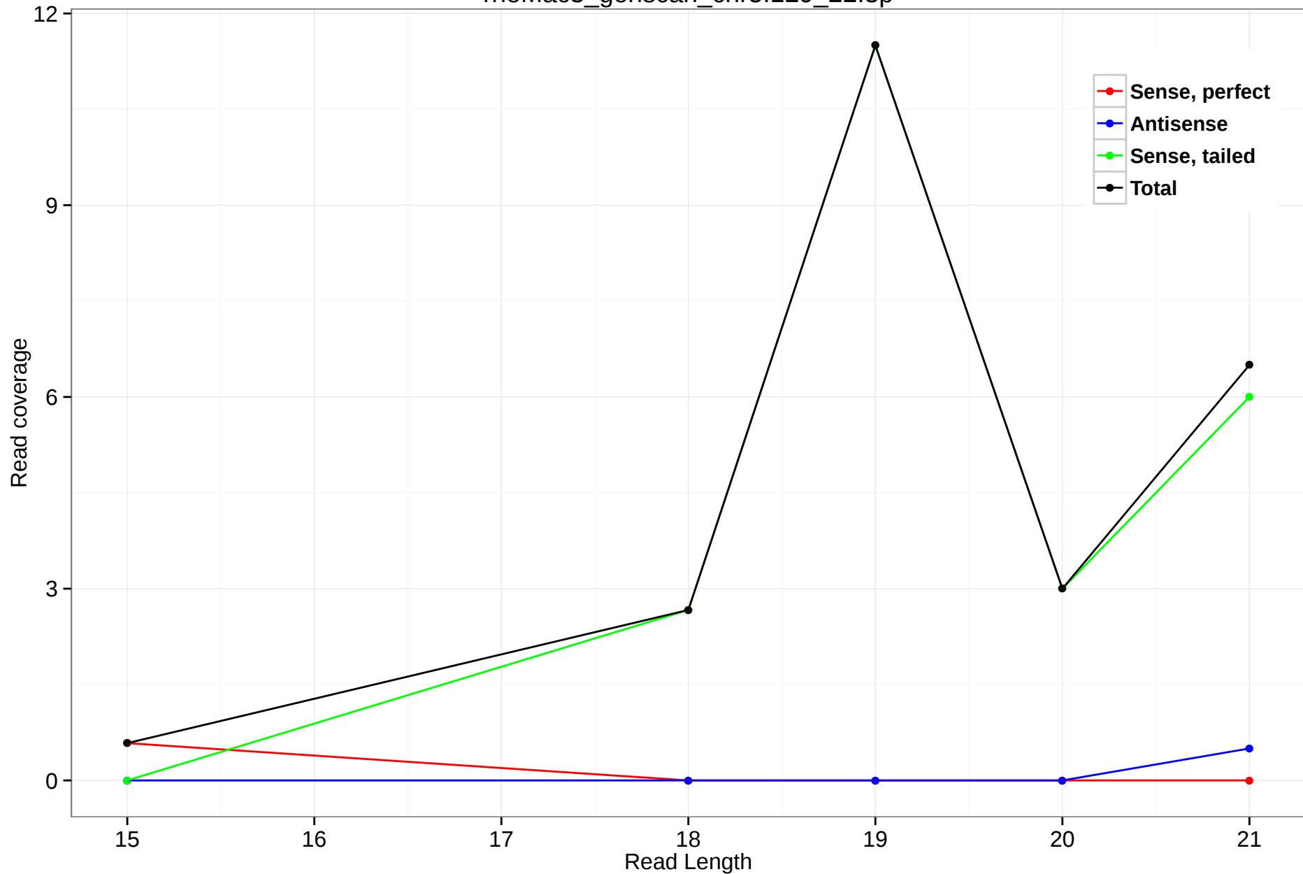
rheMac3_genscan_chr5.129_22.3p
