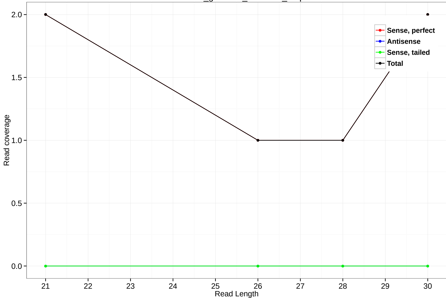
rheMac3_genscan_chr5.128_0.5p
