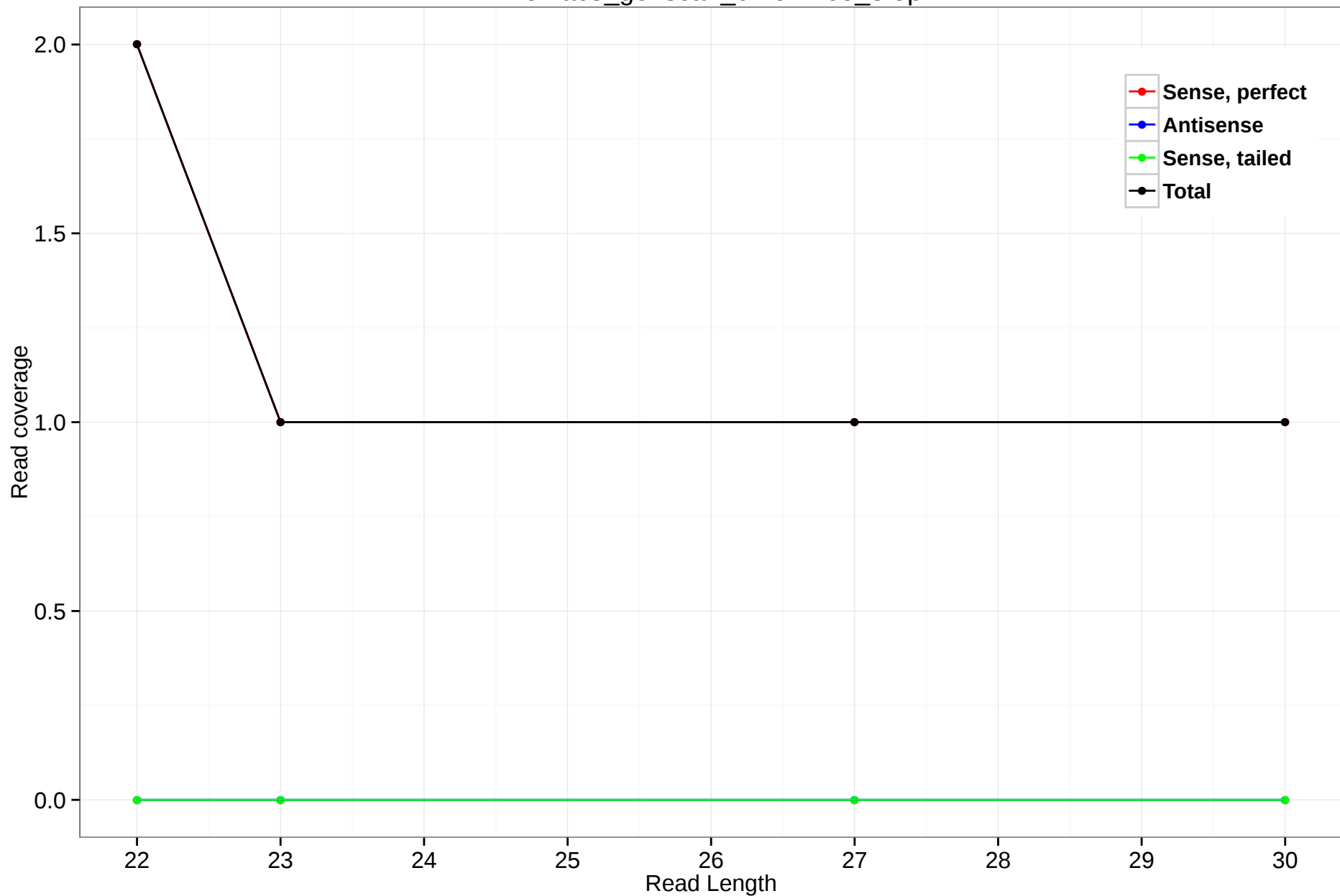
rheMac3_genscan_chr5.1263_8.5p
