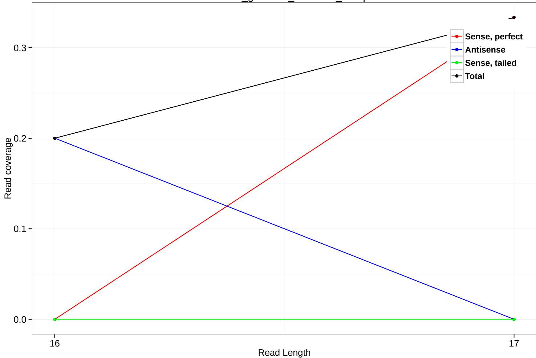
rheMac3_genscan_chr5.122_22.5p
