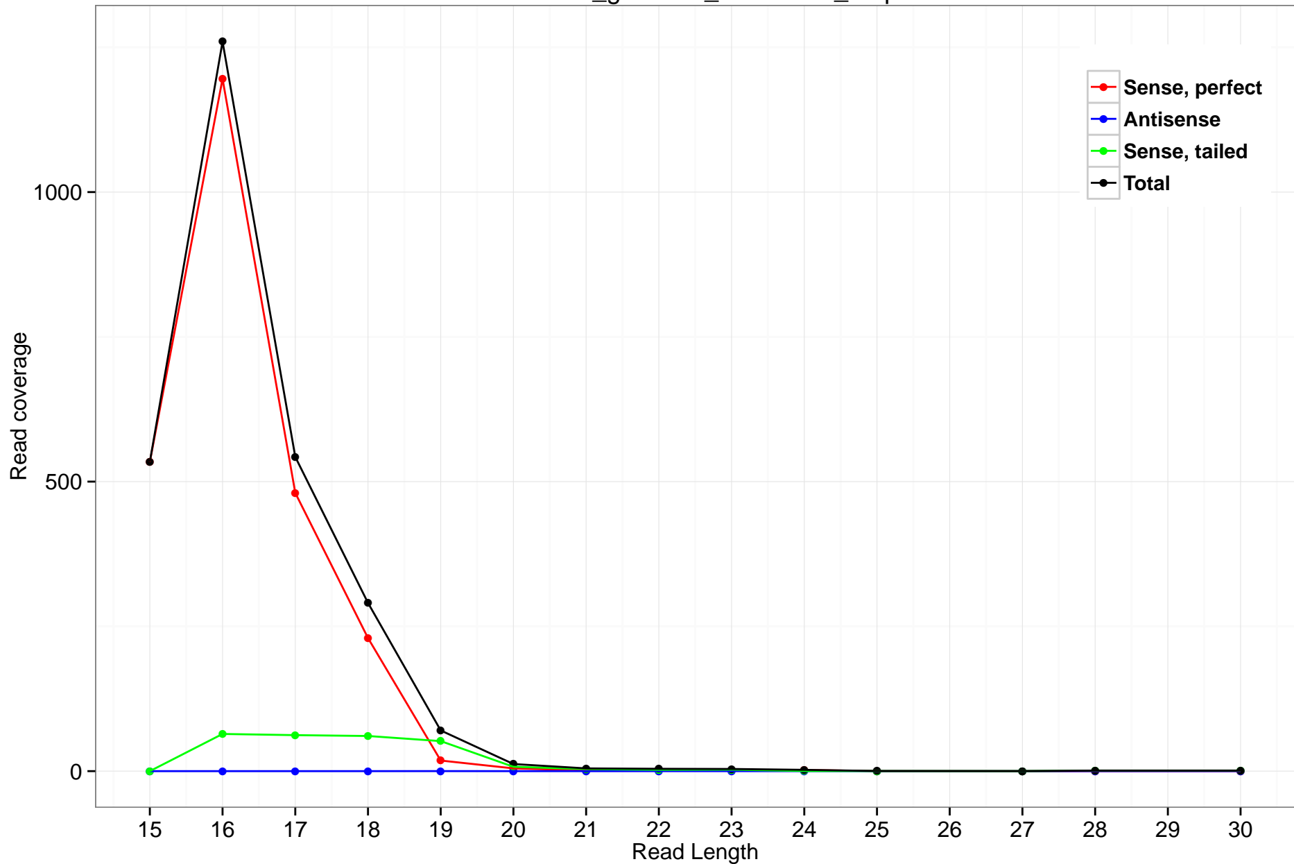
rheMac3_genscan_chr5.1226_2.5p
